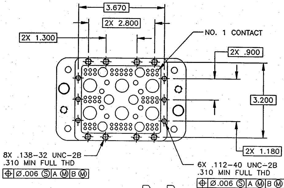
VIEW B-B (-1)
