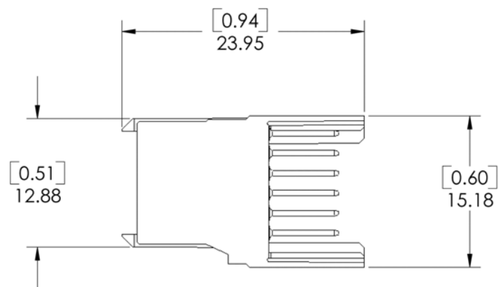
Figure 8. Adapter Connector, 311P822-FA-110-A 110 Contacts, Style A; Mates 311P822 Female Motherboard Connector to Commercial cPCI™ Daughterboard Connector
