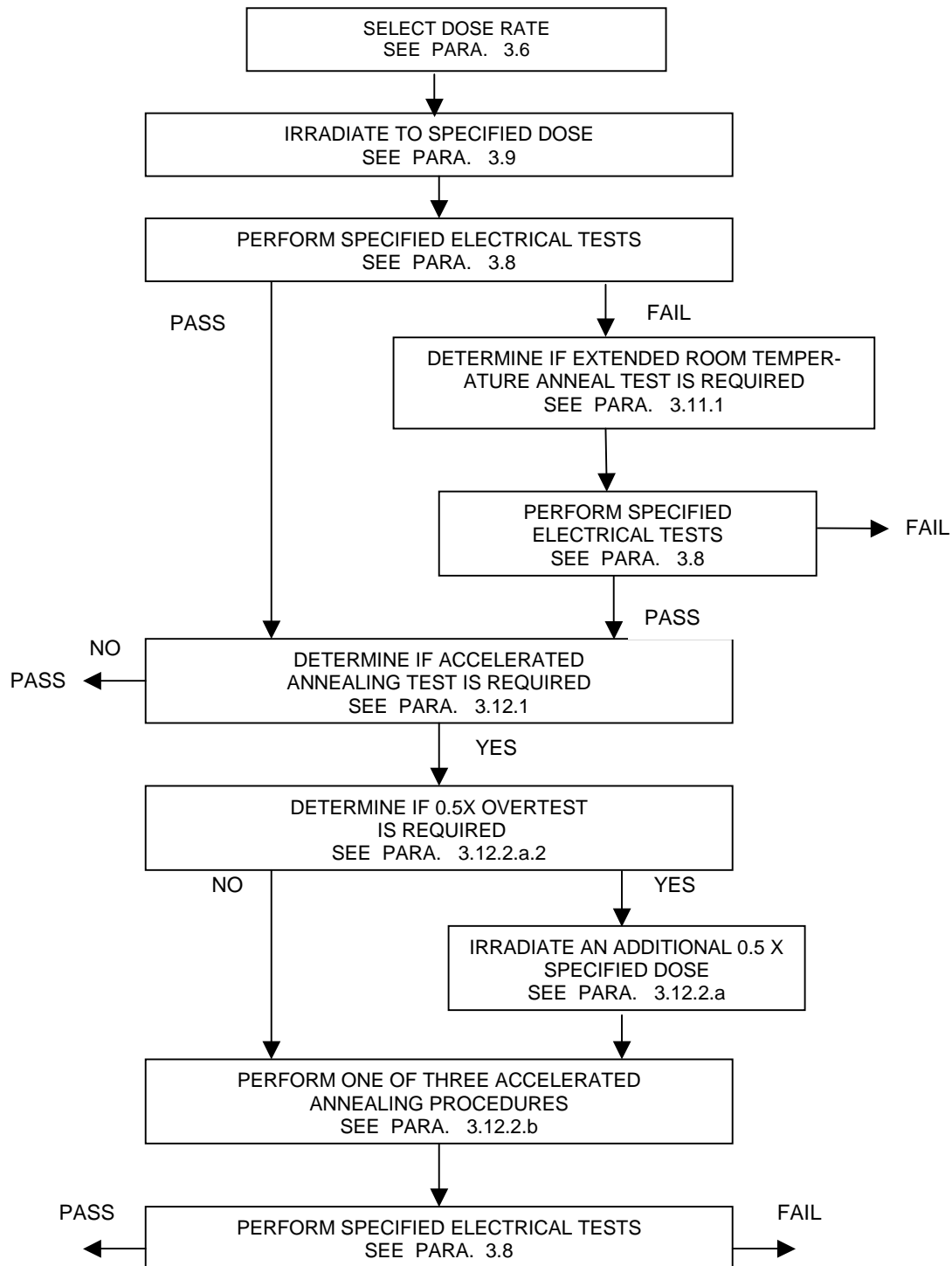
FIGURE 1019-1. Flow diagram for ionizing radiation test procedure for MOS and digital bipolar circuits.
