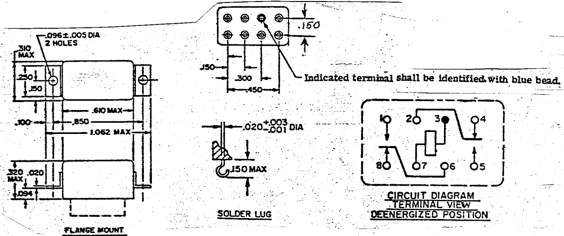
Figure 1. Configuration and circuit diagram.
