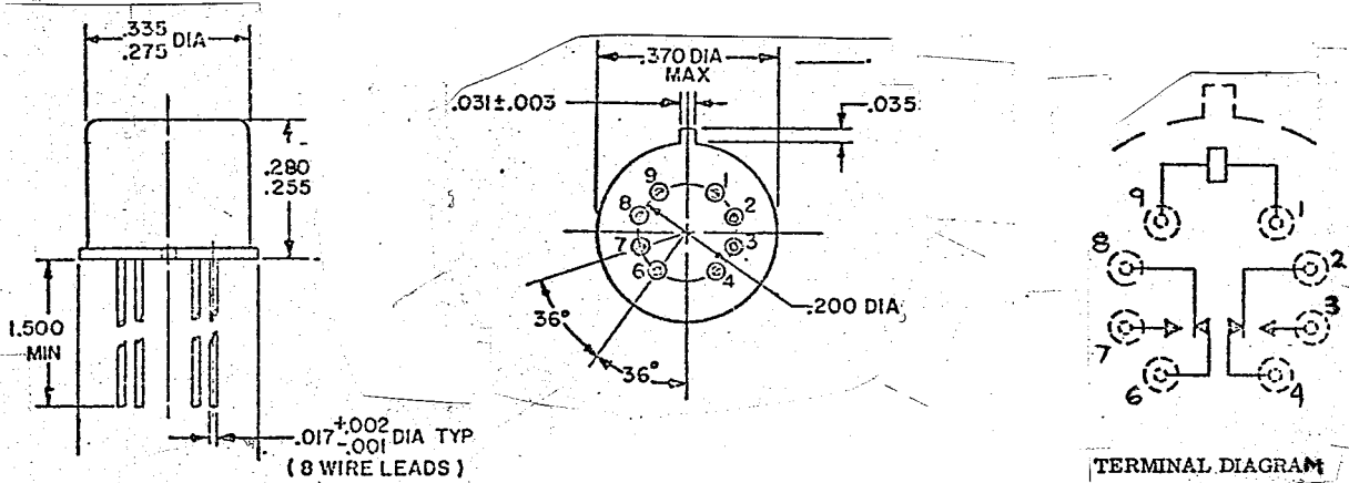
Figure 1. Configuration and circuit diagram.
