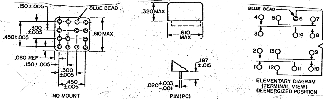
Figure 1. Configuration and circuit diagram.
