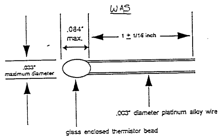
Figure 1. Physical configuration for Style A.
