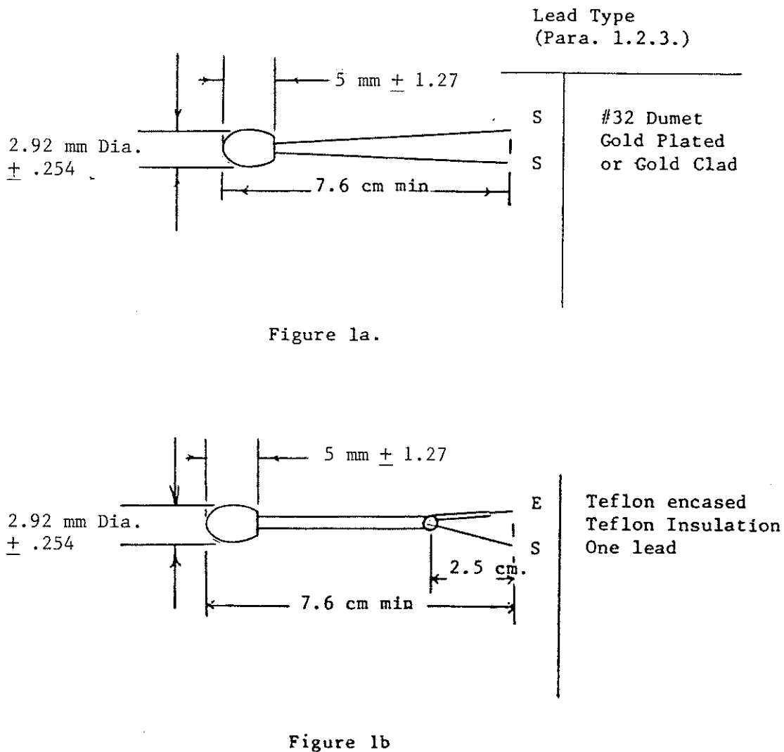
Figure 1. Thermistor Configuration
