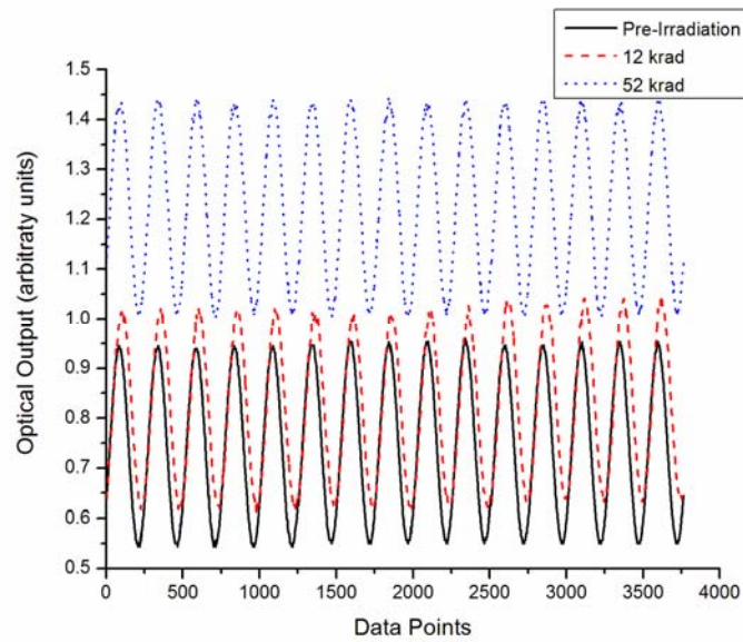
Figure 6: Modulator output pre-irradiation and at 12 krad and 52 krad exposure to gamma radiation
