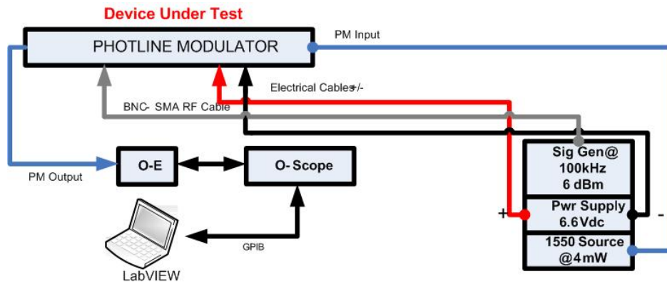
Figure 1: Modulator experimental setup
