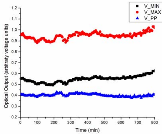
Figure 7: Modulator output during first 800 minutes of radiation test. Maximum and minimum voltage are shown in top two curves. The bottom curve is the peak-to-peak voltage difference, which remained constant throughout the remainder of the test.
