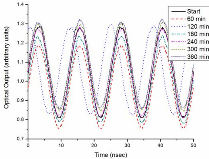
Figure 8: Modulator output after radiation test. Data were collected a month after completion of radiation test. Drift in output is similar to pre-irradiation results. No change in frequency or peak-to-peak output was observed.
