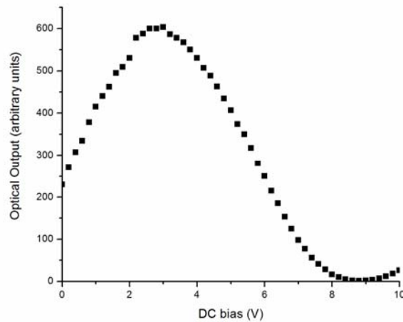
Figure 4: DC bias versus optical output from modulator with no RF bias applied
