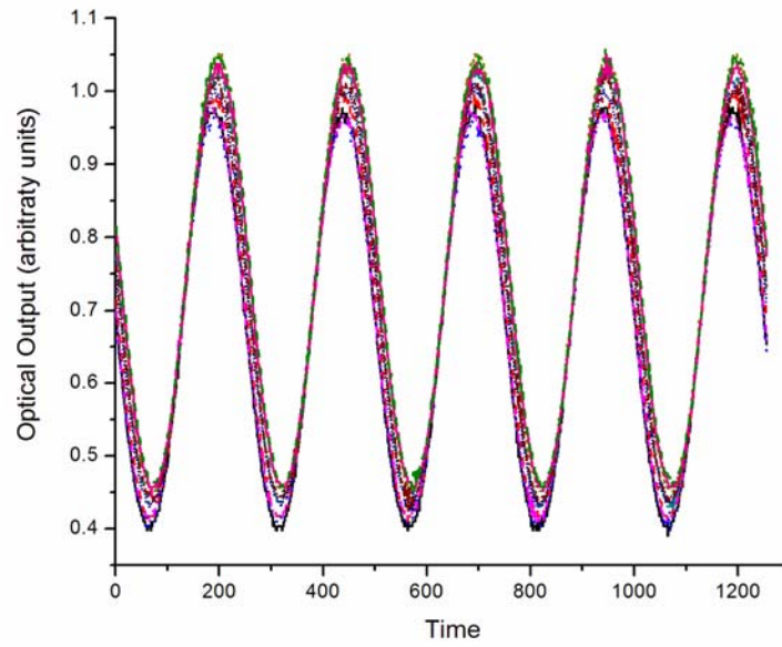
Figure 5: Benchtop test of modulator before radiation testing. Data show normal drift with no change in peak-to-peak voltage or frequency.
