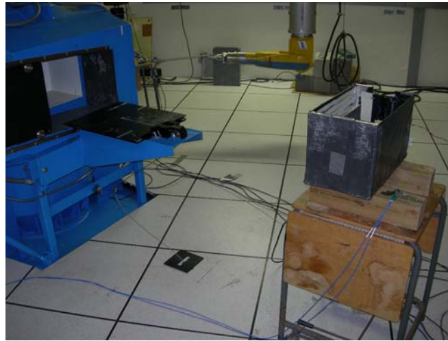
Figure 3: LiNbO 3 Modulator in radiation test cell
