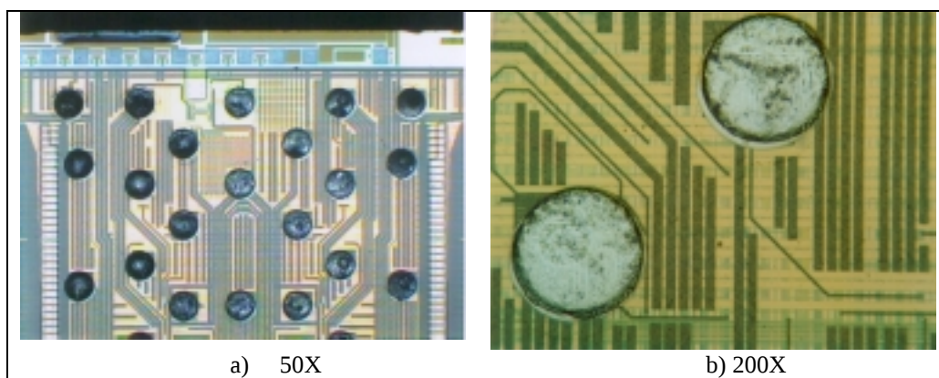
Figure 5. Close-up of the solder balls on the die.
