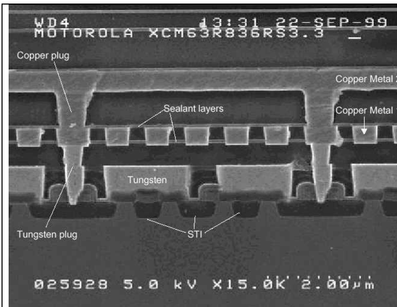
Figure 12. 15000X. Cross-section through lower metal and dielectric layers.
