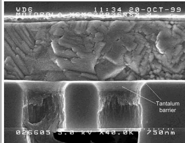
Figure 13. SEM 40000X. Cross-section through metal track high- lighting copper grain structure and tantalum barrier metal.
