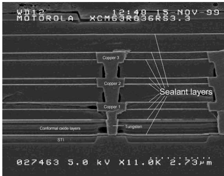
Figure 19. SEM 11000X. Cross-section of edge seal structure. (Dielectric fault is etching artifact).
