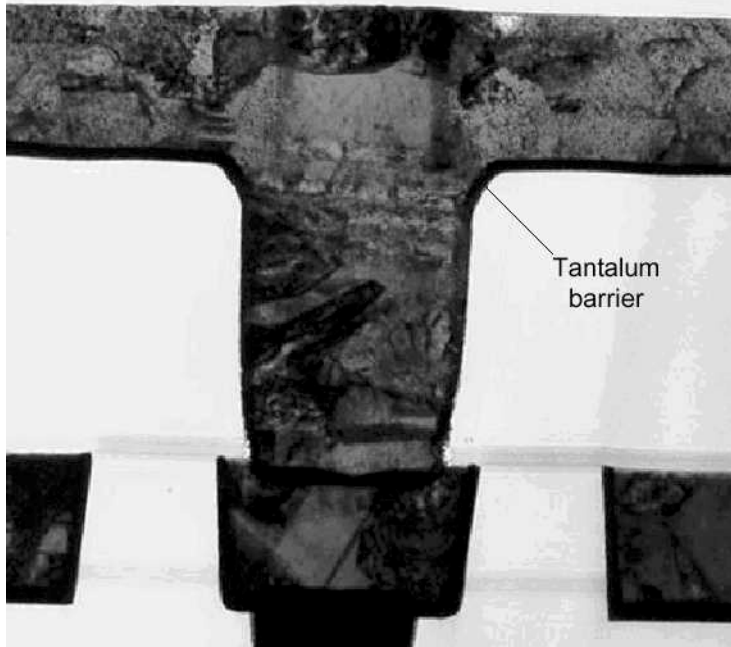
Figure 14. TEM ~40000X. TEM image of cross-section showing copper grain structure and tantalum liner.
