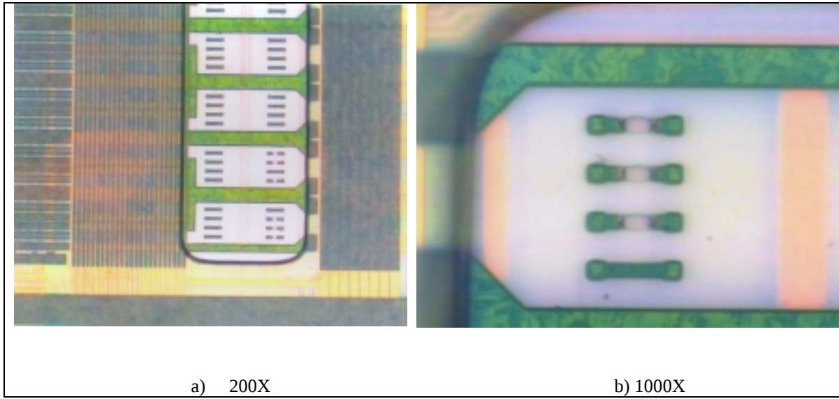
Figure 7. Close-up of the fuses on the die surface.
