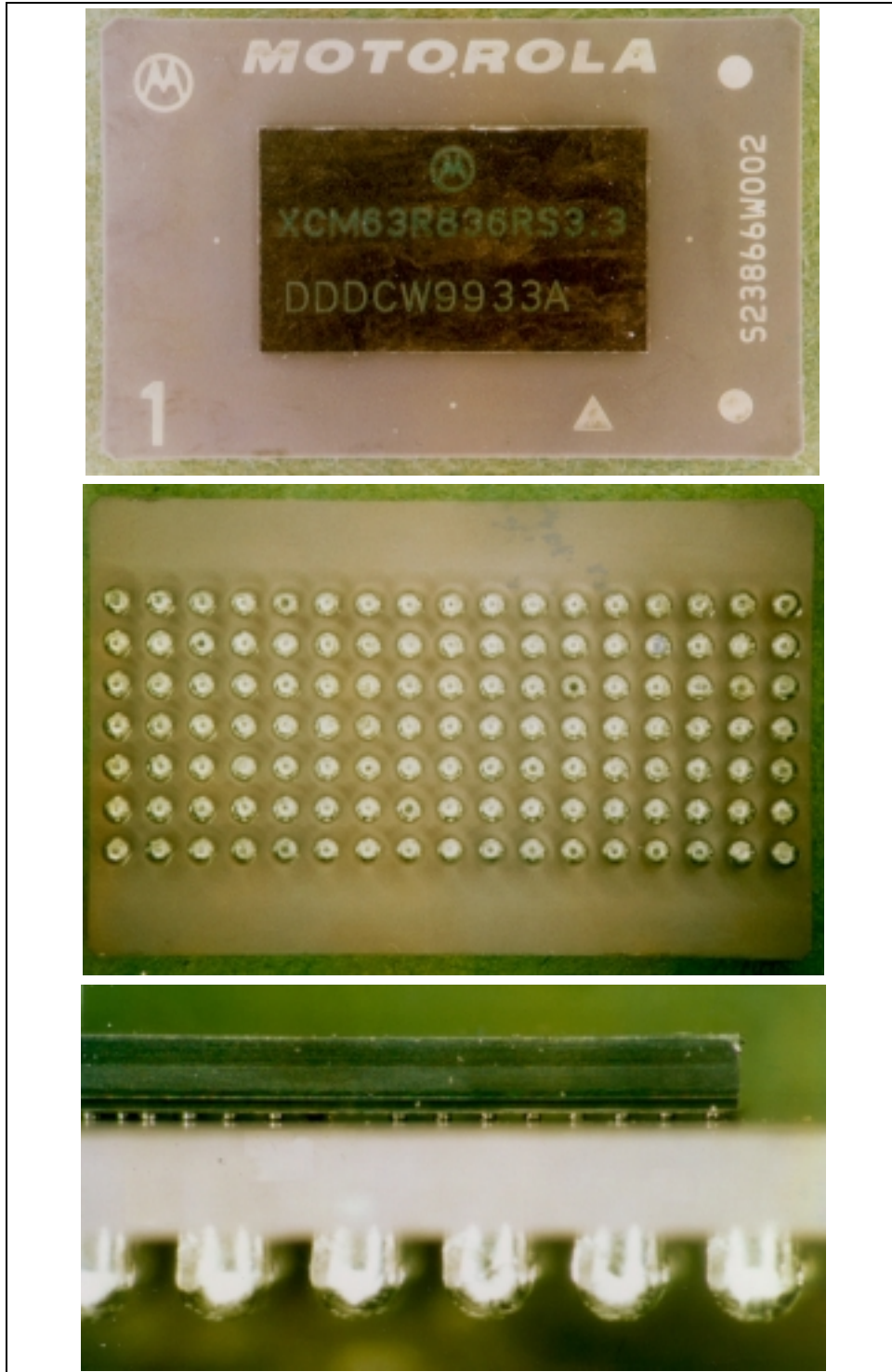
Figure 1. External top, bottom, and side aspects of the part.
