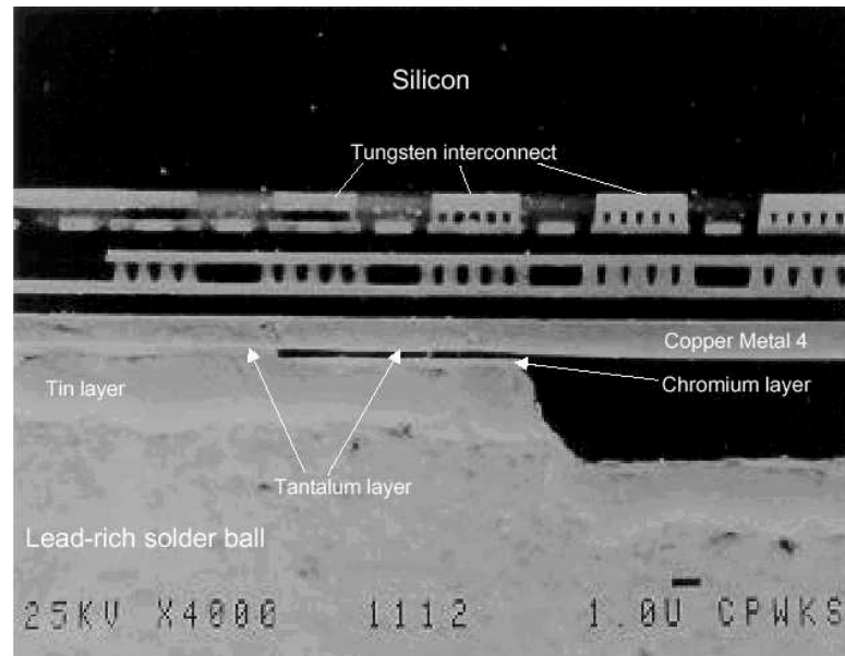
Figure 9. SEM 4000X. Cross-section through solder ball and pad metallization.
