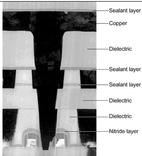
Figure 16. TEM ~30000X. TEM image showing dielectric layers and sealant layers. Copper Sealant layer
