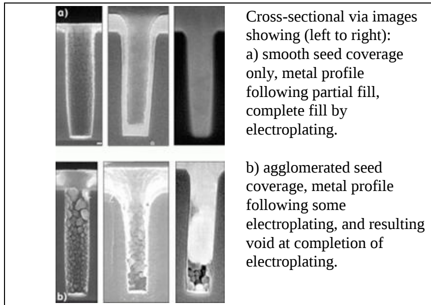
Figure 3. Normal (a) and defect-generating (b) via filling processes.
