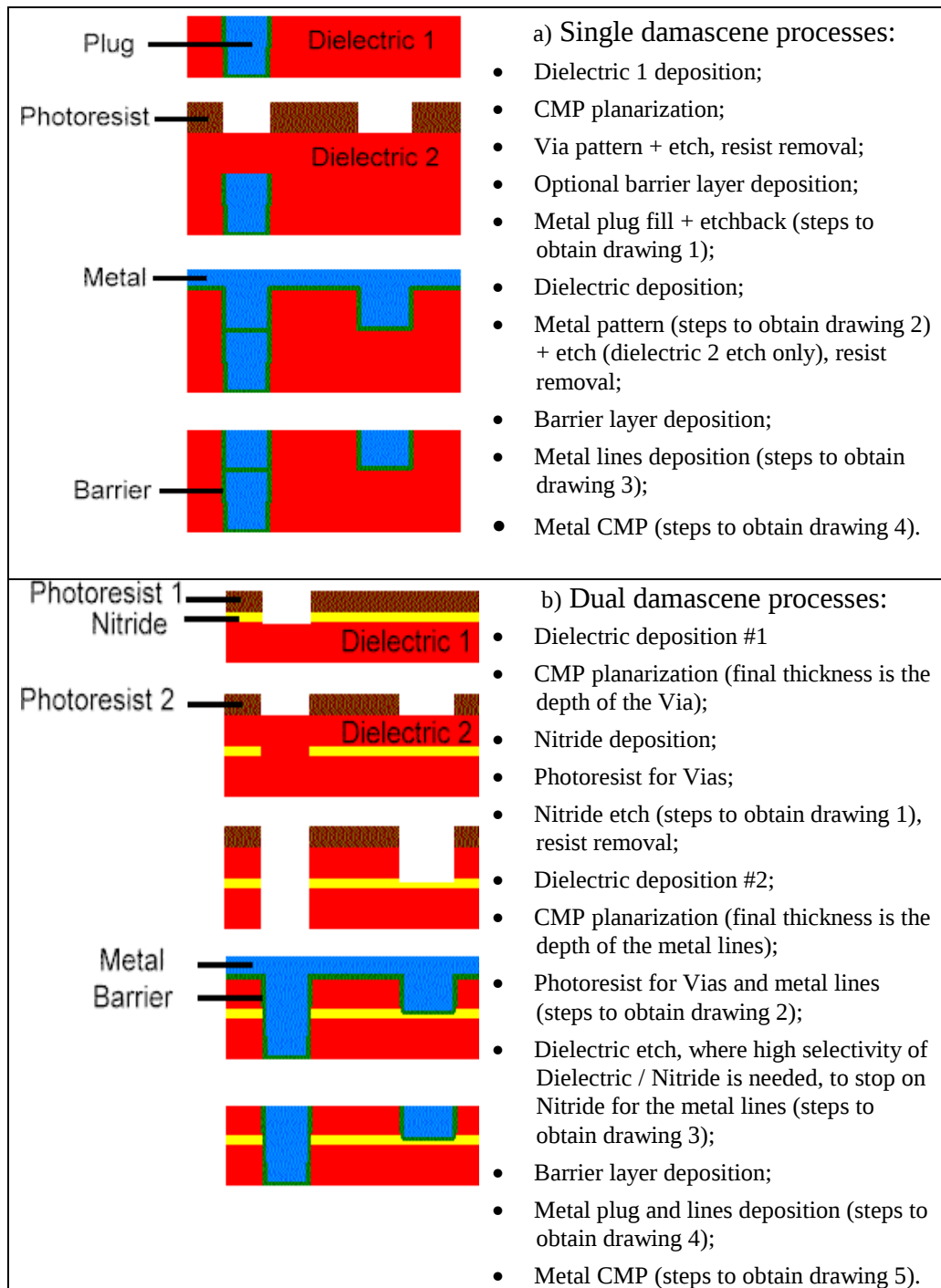
Figure 2. Single (a) and dual (b) damascene processes.
