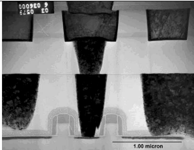
Figure 18. TEM ~39,800X. Cross-section through transistors and contacts.
