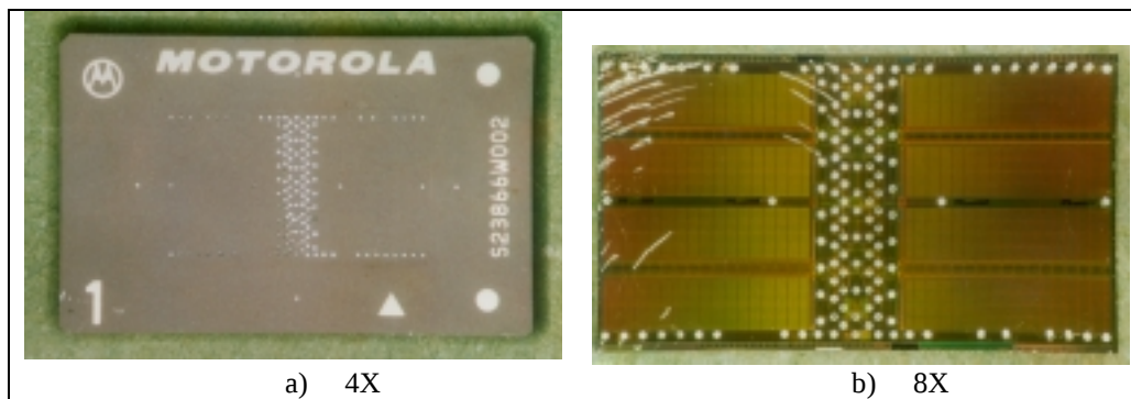
Figure 4. Ceramic substrate (a) and die (b) after the part deprocessing. The solder "threads" on the die surface (left top corner) were formed during desoldering. These "threads" were located on the polyimide film and did not cause any damage to the die.
