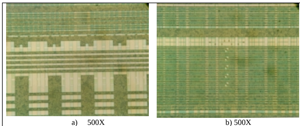
Figure 6. Aspects of the top level copper metallization.
