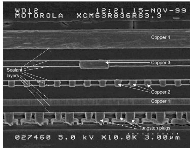
Figure 11. SEM 10000X. Cross-section through die metallization structure.
