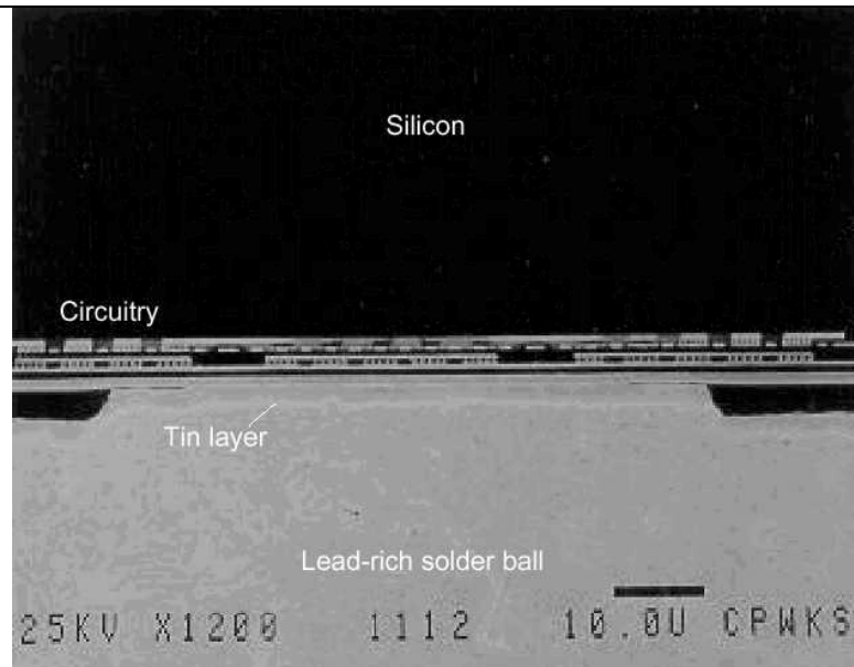
Figure 8. SEM 1200X. Cross-section through solder ball contact to pad metal.
