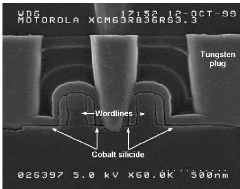
Figure 17. SEM 60000X. Cross-section through transistors and contacts.
