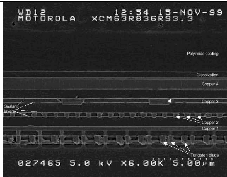
Figure 10. SEM 6000X. Cross-section through copper and tungsten metallization structure.
