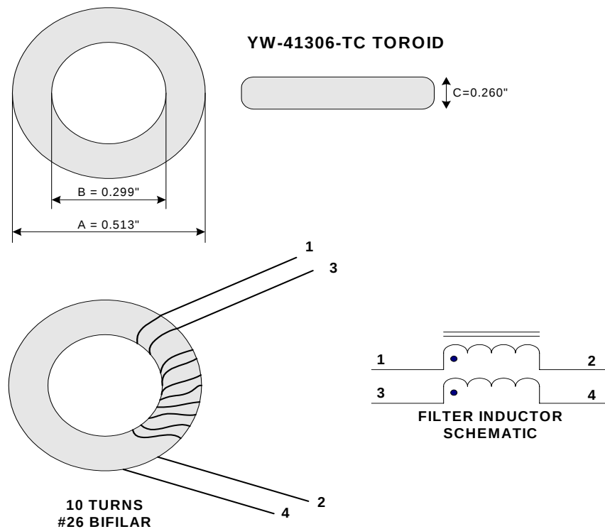
Figure 1. Filter Inductor
