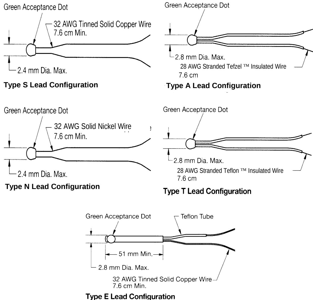
Figure 1. Thermistor configuration.
