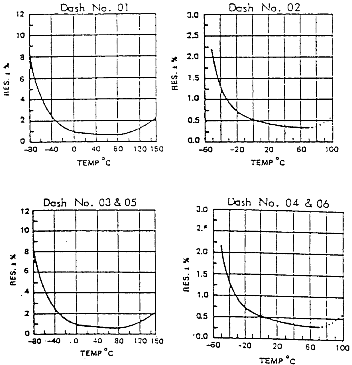
Figure 2. Resistance tolerance curves (Page 1 of 2).
