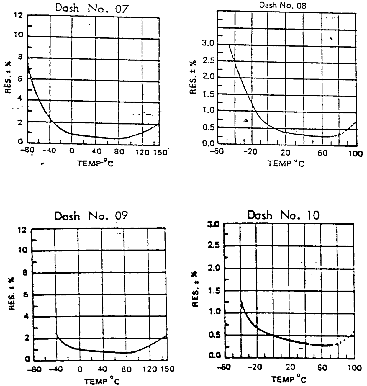
Figure 2. Resistance tolerance curves (Page 2 of 2).
