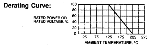
Figure 2. - Resistor derating.
