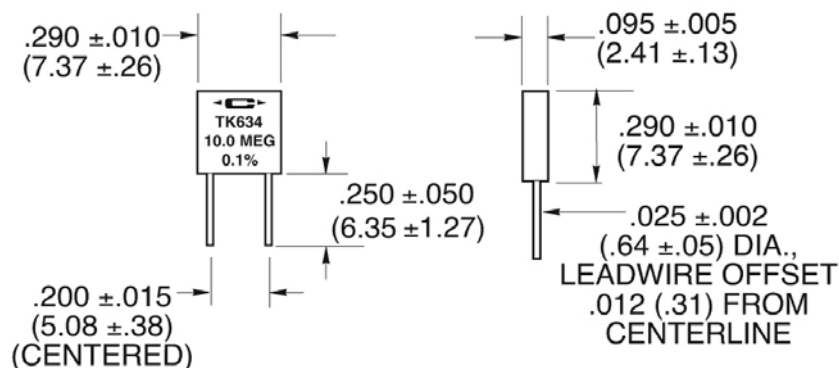
Figure 1. - Resistor outline drawing - inches (mm).
