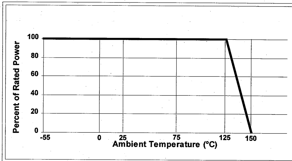
Figure 2. - Resistor derating .
