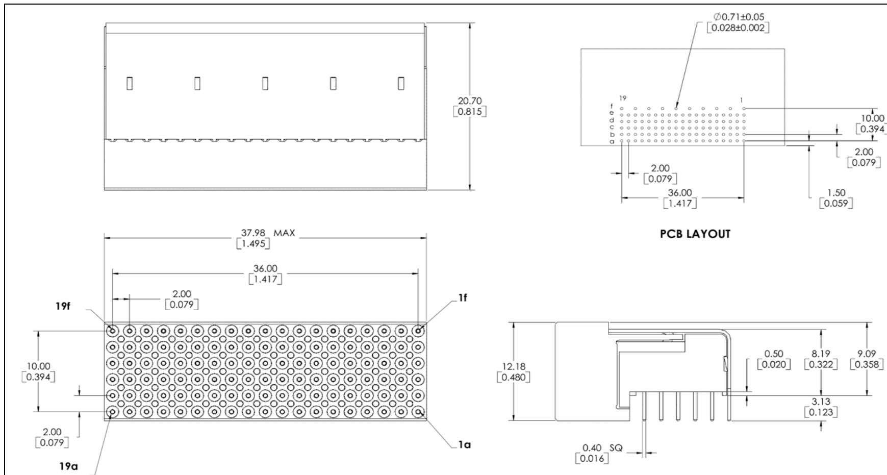
Figure 7. Male Daughterboard Connector, 311P822-MC-095-B(X)-D(X) Right Angle, 95 Pin Contacts, Style B
