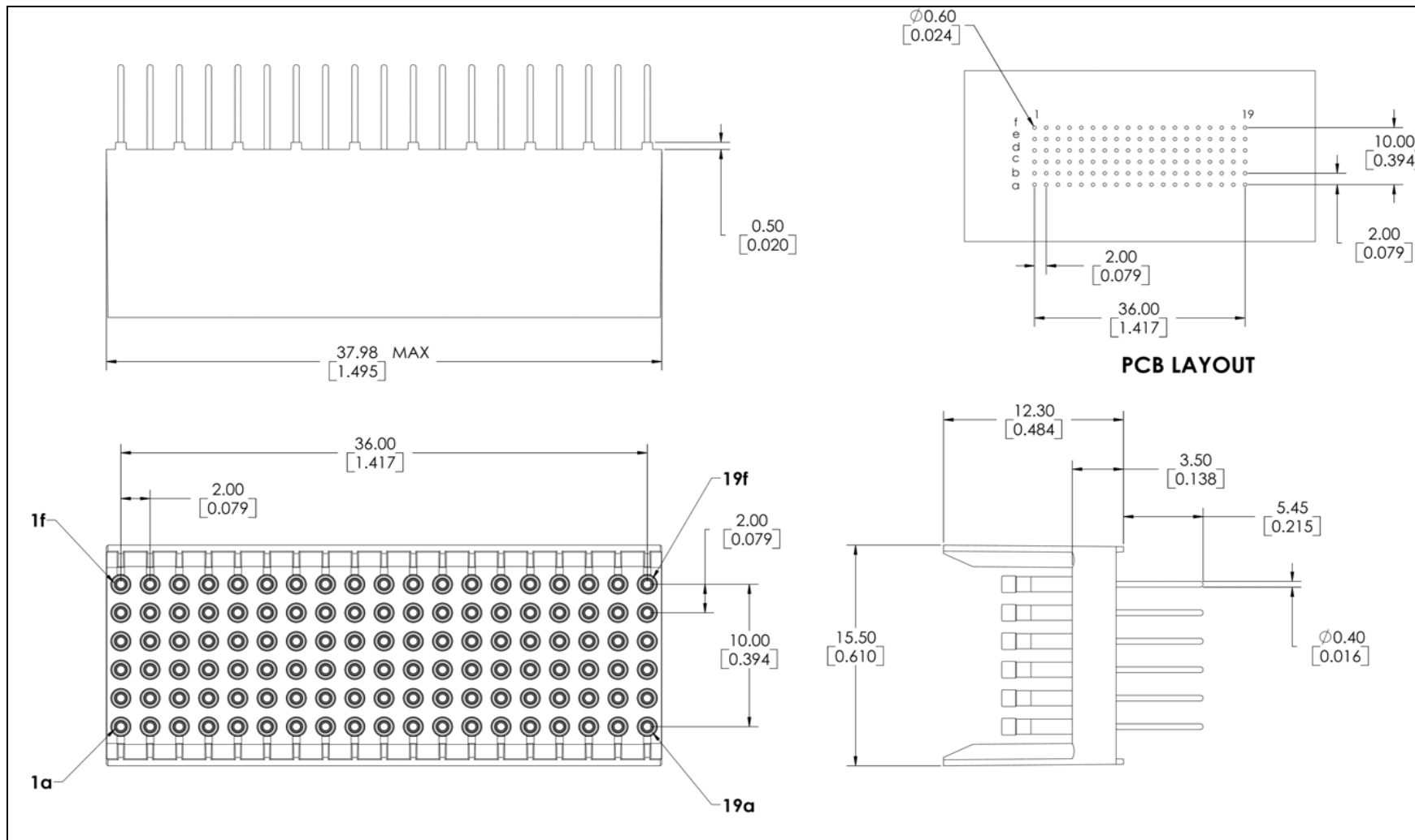
Figure 6. Female Motherboard Backplane Connector, 311P822-FC-095-B(X)-D(X) 95 Socket Contacts, Style B
