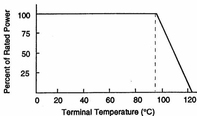
Figure 2. Derating
