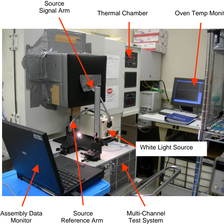
Figure 3: Setup of Thermal Cycling Testing on LOLA EM Assemblies
