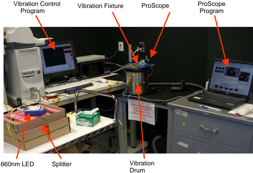
Figure 2: Setup of Random Vibration Testing on LOLA EM Assemblies
