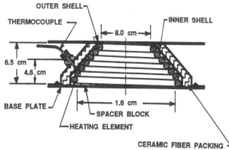
FIGURE 4. Conical Heater
