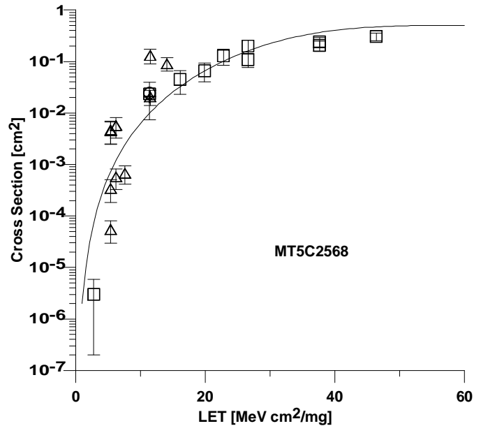
Figure 3. The SEU vs. LET cross section curve for a typical MT5C2568 SRAM. Triangles are points taken at TAM. Circles and squares were taken at BNL. The error bars are estimated from Poisson counting statistics.
