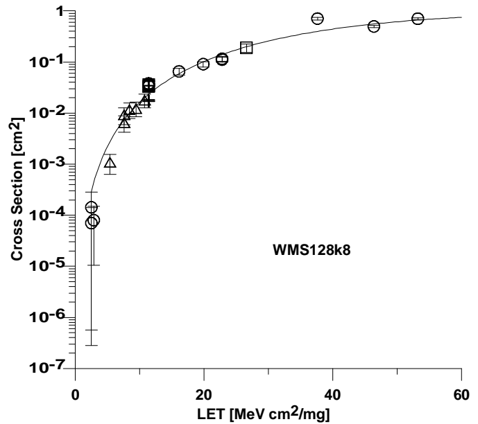
Figure 2. The SEU vs. LET cross section curve for a typical WMS128K8 SRAM. Triangles are points taken at TAM. Circles and squares were taken at BNL. The error bars are estimated from Poisson counting statistics.
