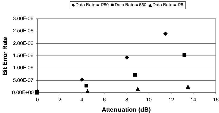
Fig. 5. Bit error rate as a function of attenuation for different data transmission rates and for an angle of incidence of 90 degrees. Clearly, the error rate increases with increase attenuation and with increasing transmission rate.
