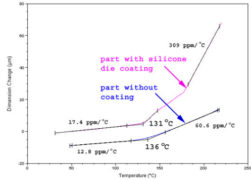
Fig. 9. Thermo-mechanical measurements of the molding compound and plastic packages used in sensors encapsulated in DIP-16 packages.
