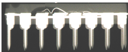
Fig. 7. Side X-ray view of the part.
