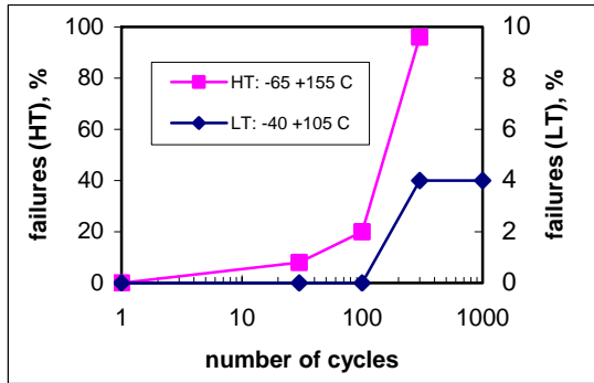
Fig. 8. Proportion of failures (%) versus number of temperature cycles.
