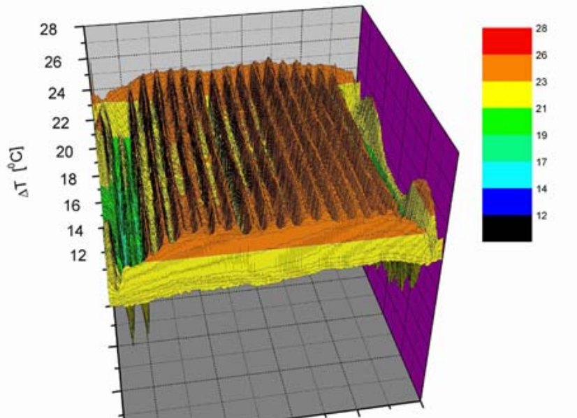
Figure 11. Thermal image showing individual emitters relative temperature; from [4]
