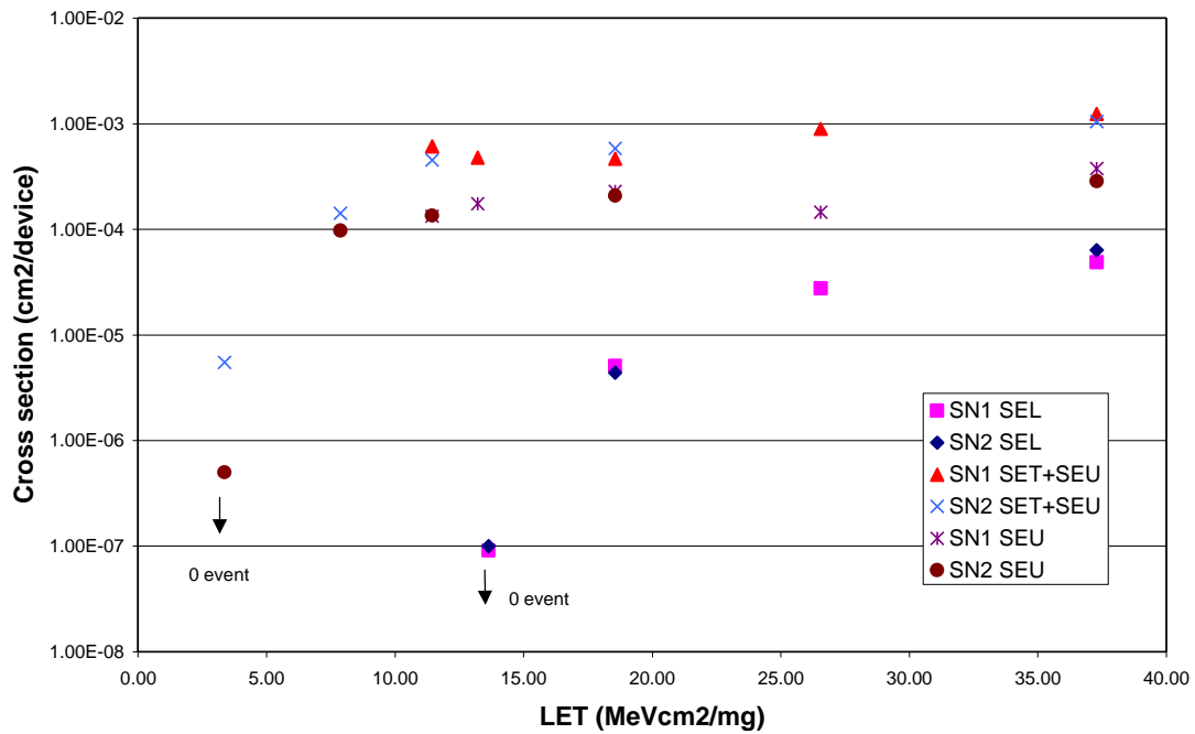
Figure 1: SEU and SEL cross section.
