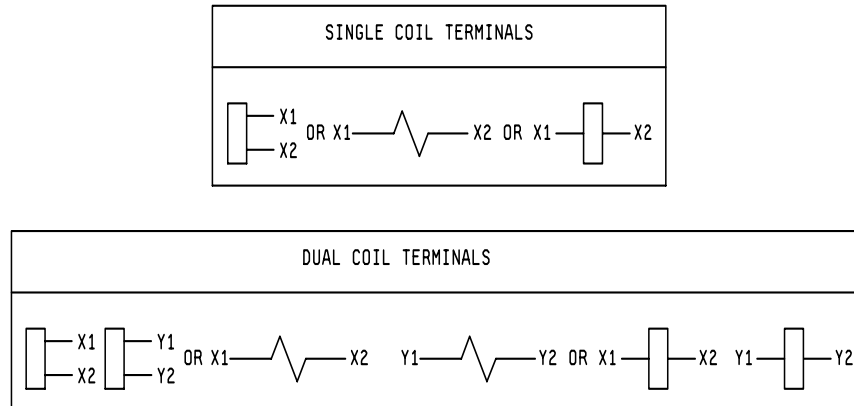
FIGURE 1. Symbols and marking for terminals.
