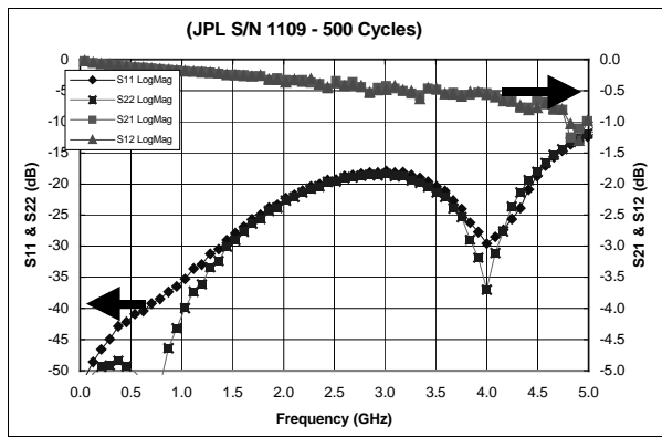
b) After 500 Cycles (-55°C to 125°C)
