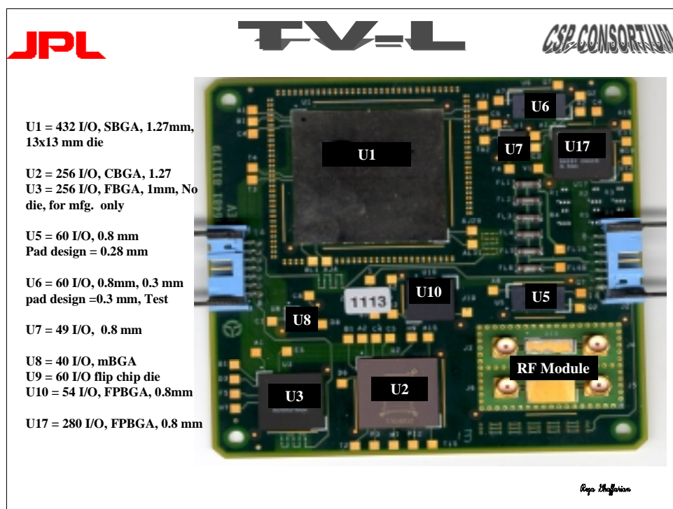
Figure 3 The assembled TV-L with numerous CSP and BGA packages and an RF module
