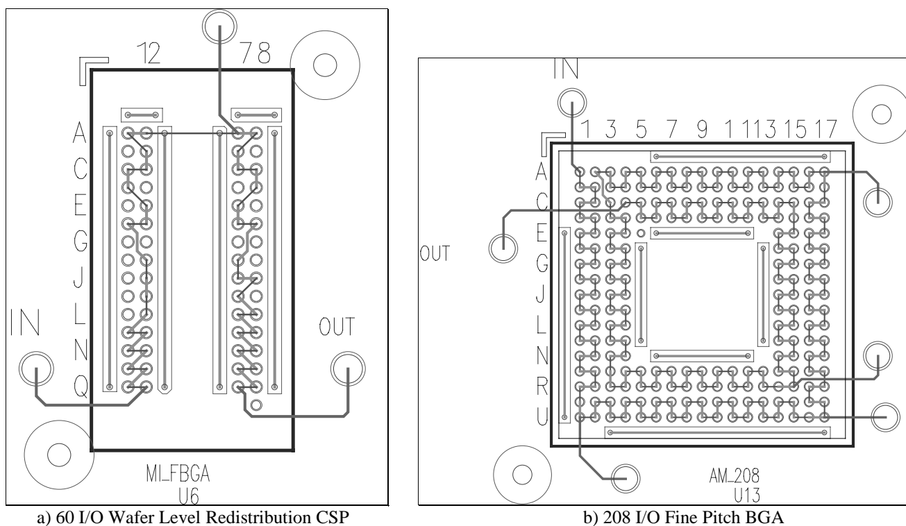
Figure 2 Package and board daisy chain patterns for two representative packages and probing points for failure diagnostics
