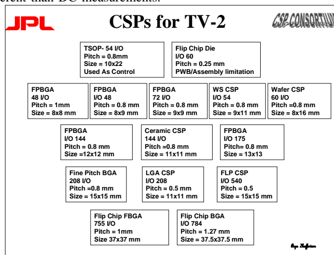
Figure 1 Description of fifteen different CSPs used in TV-2
