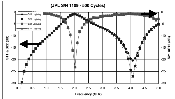
b) After 500 Cycles (-55°C to 125°C)
