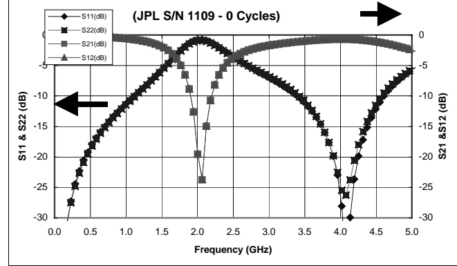
a) As Assembled
