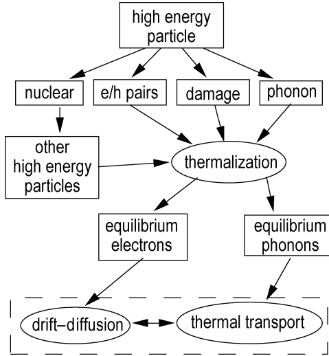
Fig. 1. Schematic representation of the relationship of thermal effects and other physical phenomena that are important to device behavior during radiation events. The dashed box represents the models for typical device simulation.
