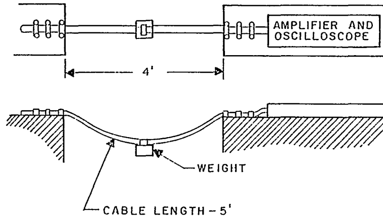
FIGURE 9. Equipment setup.
