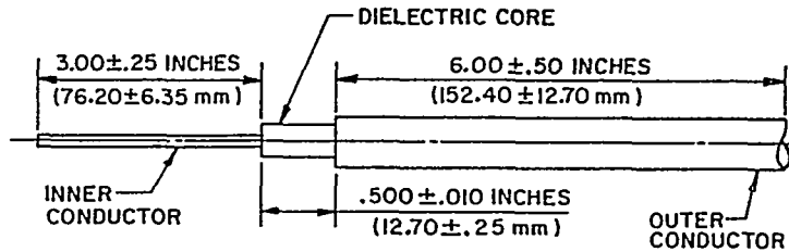
FIGURE 2. Stripping dimensions for semi-rigid cables.
