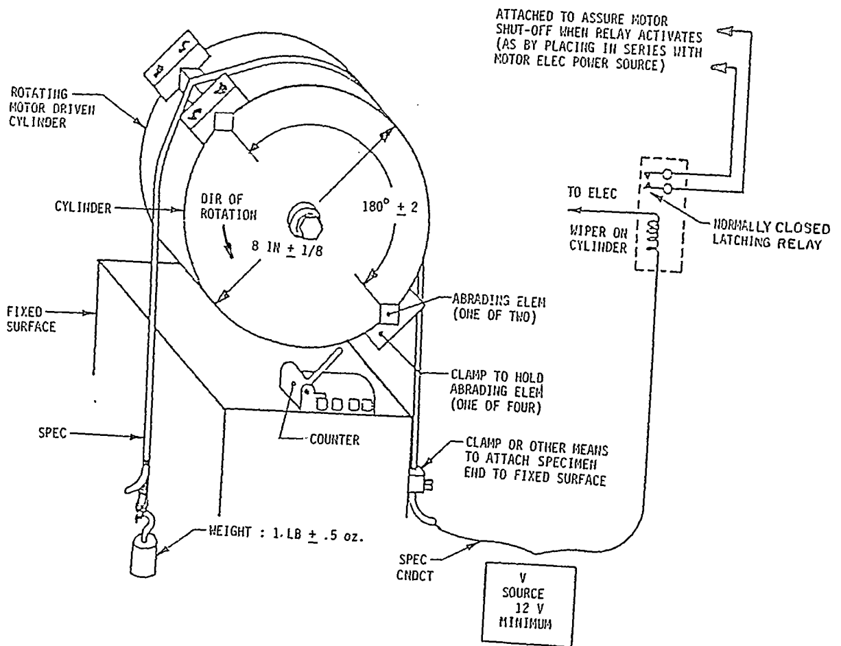
FIGURE 13. Diagram of abrading machine for the abrasion resistance test.
