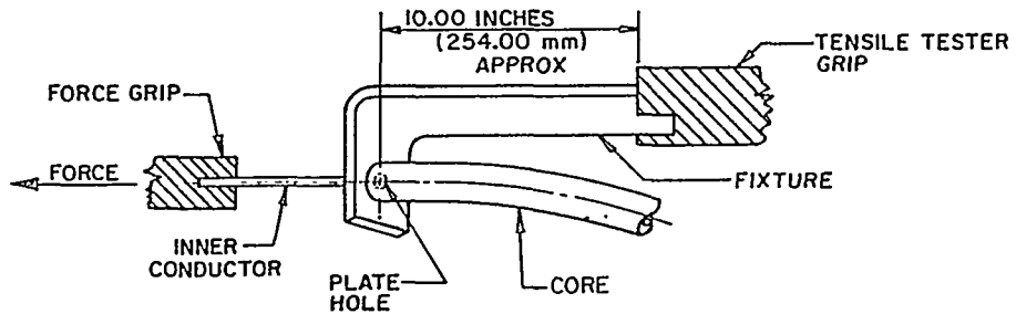
FIGURE 3. Typical test fixture for use with flexible cables.
