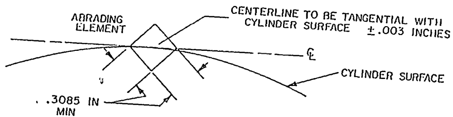
FIGURE 13. Diagram of abrading machine for the abrasion resistance test.
