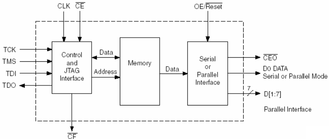
Figure 7: XC18V04-series PROM block diagram
