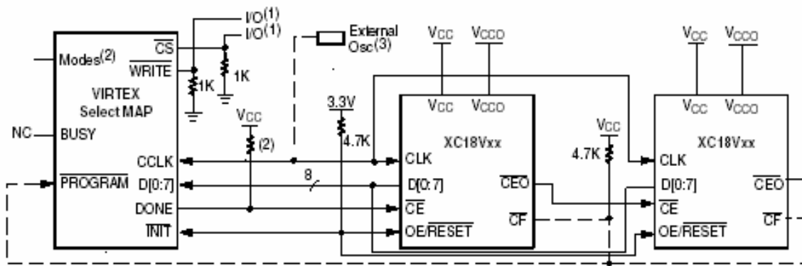
Figure 8: Cascading multiple EEPROMs (with the FPGA in SelectMAP Mode).
