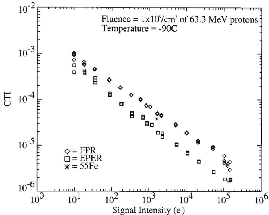
Figure 16 EPER overestimates the CTE at -90^\circ\text{C} because the longer emission time constant means that charge is released over many pixels, and even beyond the practical over-scan. Also, a small amount of charge per pixel makes it difficult to recover signal from the noise.
