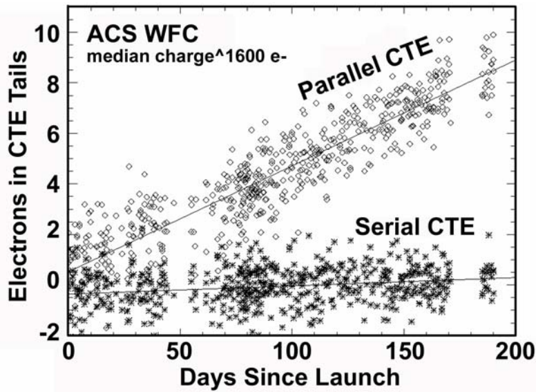
Figure 4 Advanced Camera for Surveys (ACS) Wide Field Camera (WFC) is showing significant CTE degradation as measured using cosmic ray tails. From [Reis02]. In another HST instrument (the Wide Field Camera 2 (WFC2)), the CTE has decreased 15 – 40% from 1991-1999, depending on the sky background level [Whit02]. Note that HST is a heavily shielded low earth orbit (LEO) application. (Parallel CTE is also referred to as vertical CTE, and serial CTE is the same as horizontal CTE.)
