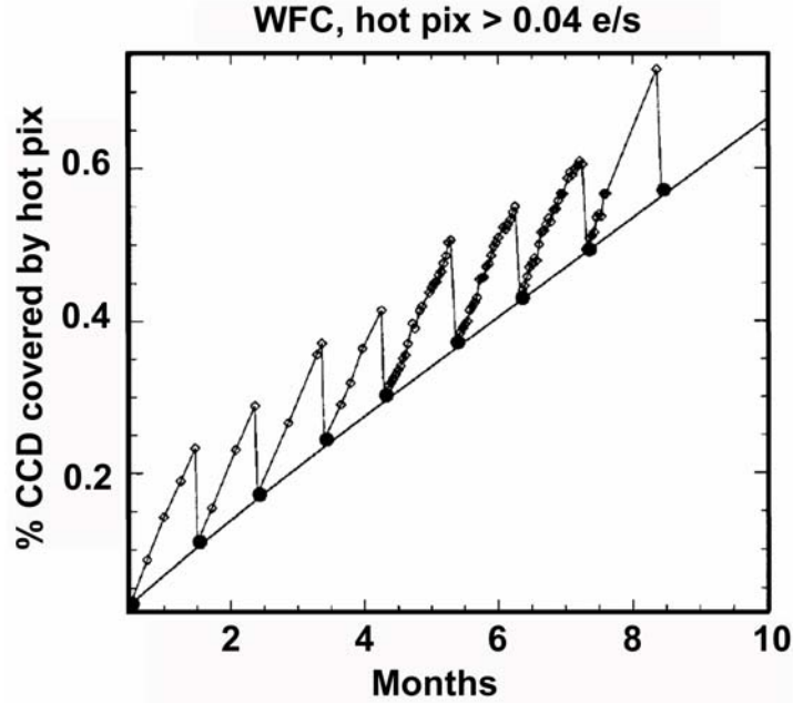
Figure 6. Hot pixel growth rates require monthly anneals that consume 10% of the observing time on the HST instruments (STIS, WFC2, ACS). From [Clam02].
