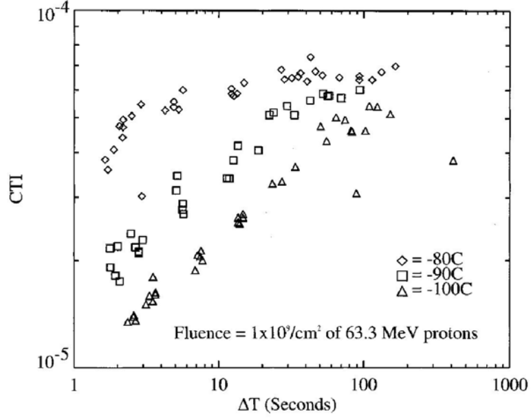
Figure 11 The charge transfer inefficiency ( CTI = 1 - CTE ) versus the time between x-ray events ( \Delta T ). CTE for images of medium density is a strong function of temperature whereas sparsely populated images are almost independent of temperature.
