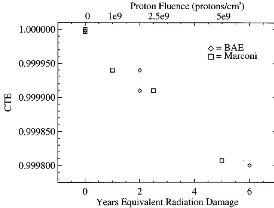
Figure 18 CTE as a function of proton fluence for 2 CCDs shown with equivalent time on orbit for HST.
