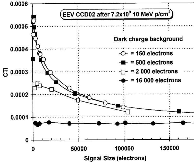
Figure 13 The charge transfer inefficiency ( CTI = 1 - CTE ) for a CCD exposed to a 10 MeV proton fluence of 7.2 \times 10^9 \text{ cm}^{-2} , corresponding to TID of 4 krad(Si). Both the CTI and the efficacy of a dark charge background in CTI reduction are a function of signal size. After [Hopk94].
