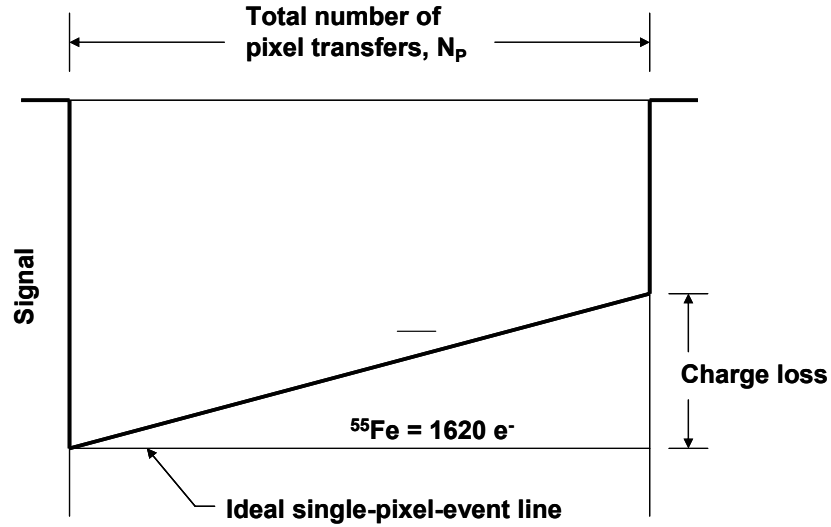
Figure 9 CTE measurement using x-ray signal charge packets.
