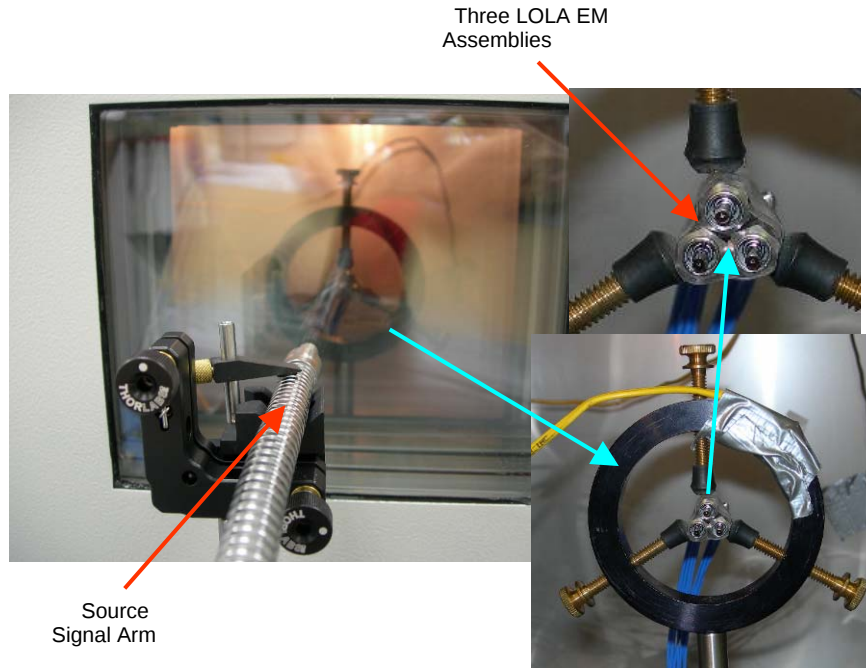
Figure 4: Setup of Three LOLA EM Assemblies in Thermal Chamber
