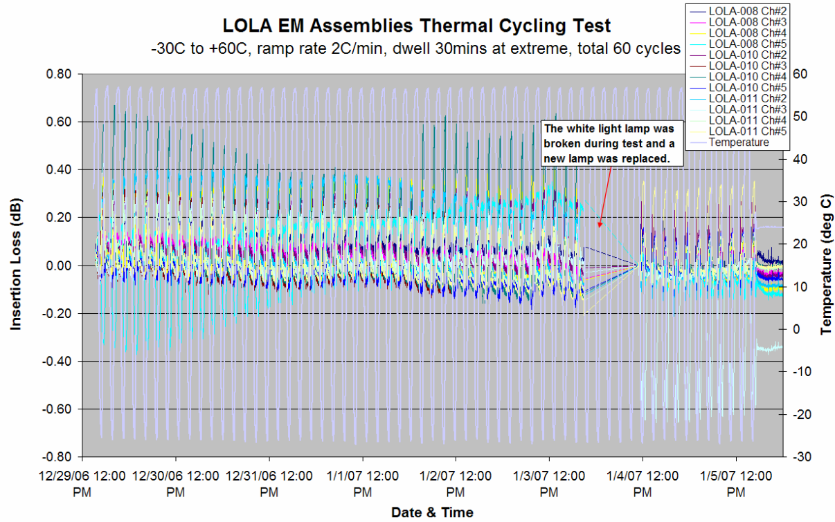
Figure 5: Thermal Cycling Test Data Plot on Three LOLA EM Assemblies
