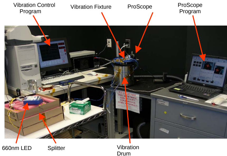
Figure 2: Setup of Random Vibration Testing on LOLA EM Assemblies
