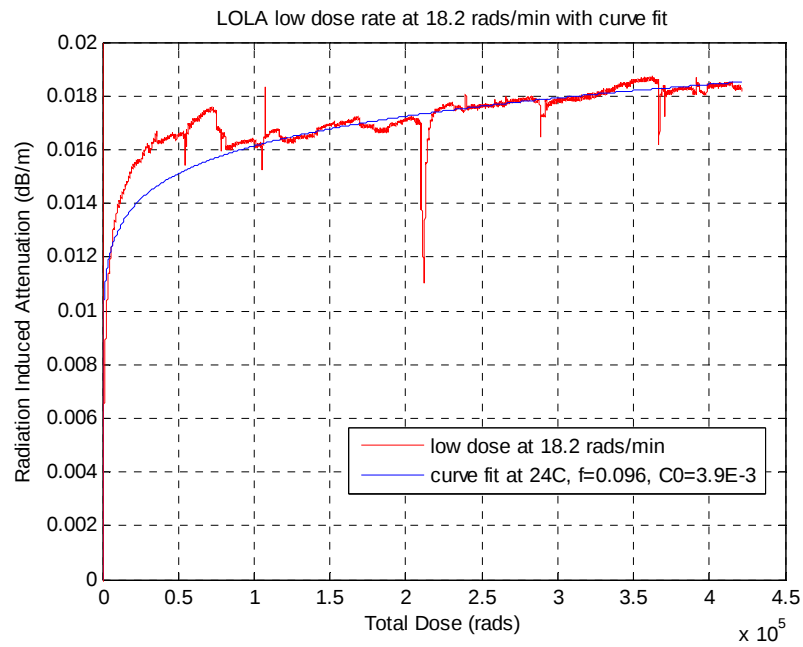
Figure 6: LOLA Fiber Cable Radiation-Induced Attenuation Data
