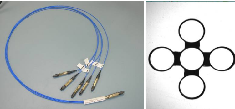
Figure 1: Completed EM LOLA Assembly with illuminated end-face.
