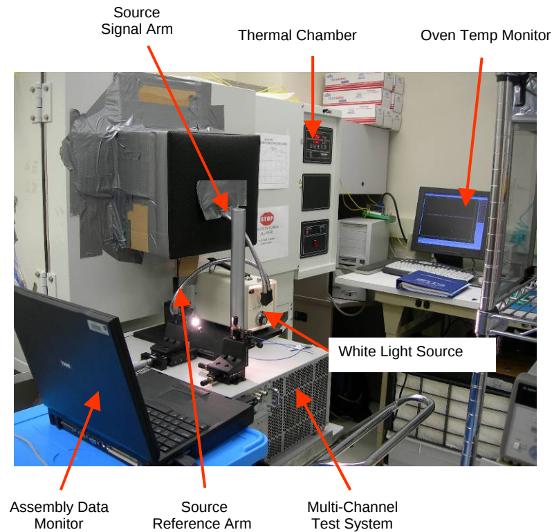
Figure 3: Setup of Thermal Cycling Testing on LOLA EM Assemblies
