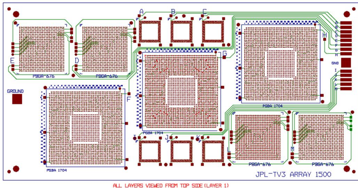
Figure 4. Test vehicle design showing combined package and board daisy-chain patterns at three locations for the 1704 I/O flip-chip BGA (FCBGA) package with 1-mm pitch and 42.5-mm 2 body size. Location and board daisy-chain patterns for PBGA 676 I/Os and 432 I/Os are also apparent in the design.
