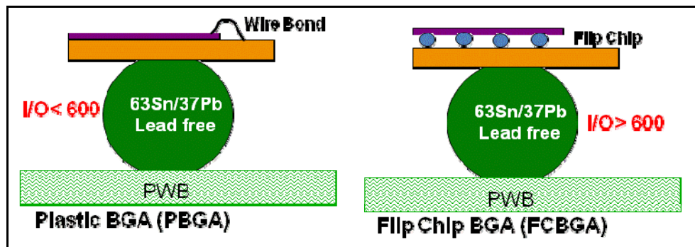
Figure 2. Typical plastic ball grid array with internal wire-bond and flip-chip die for low and high I/O package configurations, respectively.
