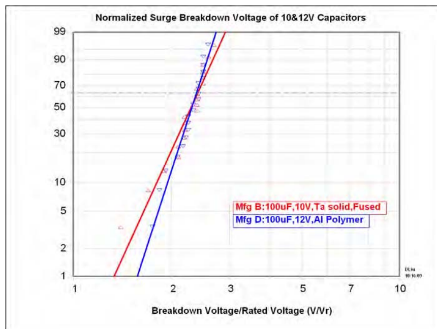
Figure 36. Normalized SSST breakdown voltages for 12V, 100 \mu F, PA capacitor made by manufacturer D and for 10V, 100 \mu F, fused \text{MnO}_2 tantalum capacitor made by manufacturer B.
