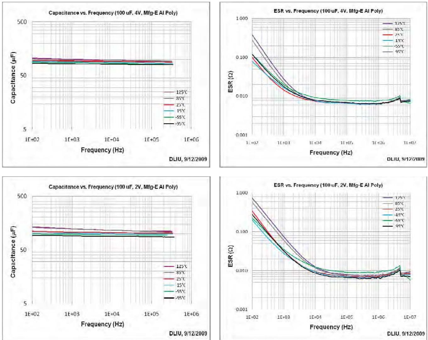
Figure 30. Capacitance and ESR vs. Frequency at Various Temperatures for 4V and 2V, 100 µF Al Capacitor made by Manufacturer E (top). Note the Measured Capacitance Shows Almost Independent to Temperature and frequency.
