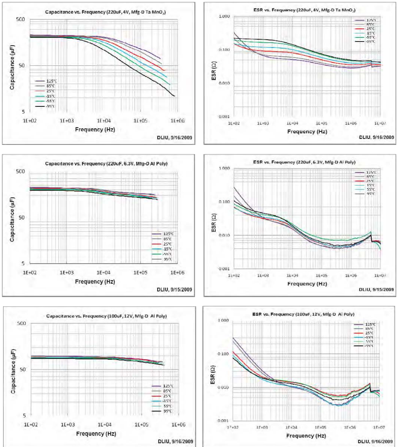
Figure 29. Capacitance and ESR vs. Frequency at Various Temperatures for 4V, 220 μF MnO 2 - Tantalum Capacitor (top), for 6.3V, 220 μF Al Polymer capacitor (middle), and for 12V, 100 μF Al Polymer Capacitors (bottom) All Made by Manufacturer D. Please Note the ESR of MnO 2 -Based is about 10 Times Higher Than Those of Al Polymer Capacitors.
