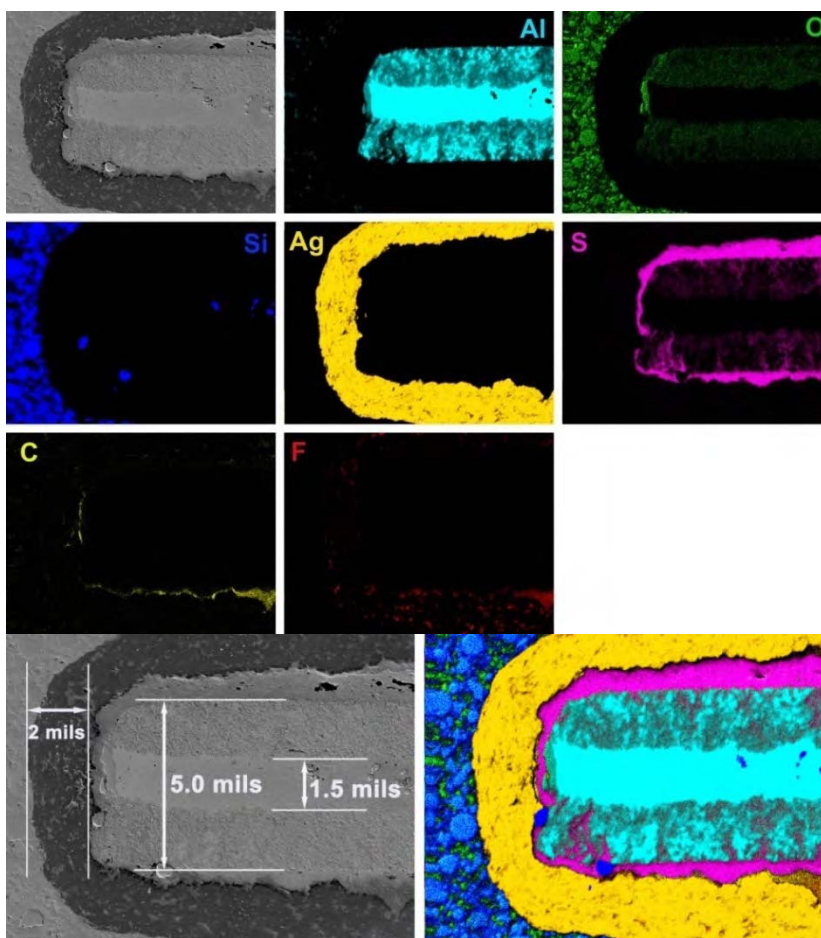
Figure 21. Cross-section SEM images and 2-dimentional EDX mapping results of a 220 \mu\text{F} , 4.0 V PA capacitor made by manufacturer D.
