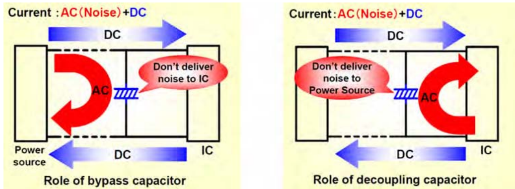
Figure 5. Bypass and decoupling applications of capacitors
