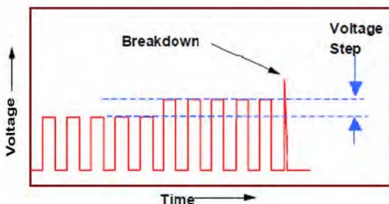
Figure 33. Increasing voltage pulse of SSST test
