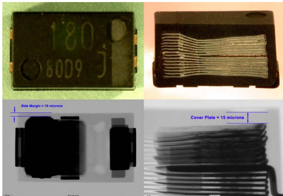
Figure 16. External and cross-section optical views as well as the top and side radiographic views of a 180 \mu\text{F} , 6.3V PA capacitor made by manufacturer A.
