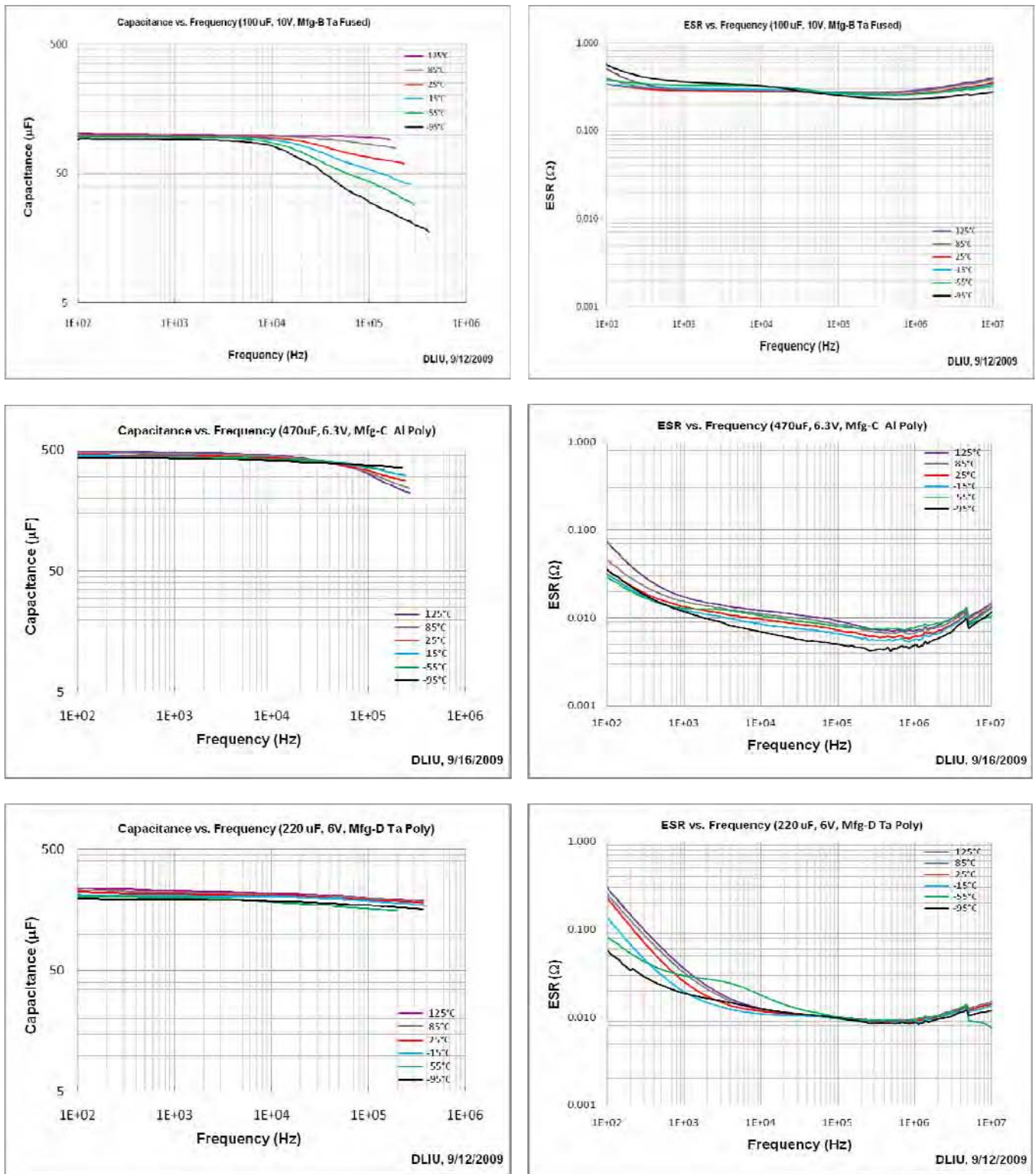
Figure 28. Capacitance and ESR vs. frequency at various temperatures for 10V, 100 \mu F fused \text{MnO}_2 -tantalum capacitor made by manufacturer B (top), for 6.3V, 470 \mu F Al polymer capacitor made by manufacturer C (middle), and for 6.0V, 220 \mu F Ta polymer capacitors made by manufacturer D (this capacitor has a measured ESR of 9 m \Omega at 100 kHz as specified (bottom)).
