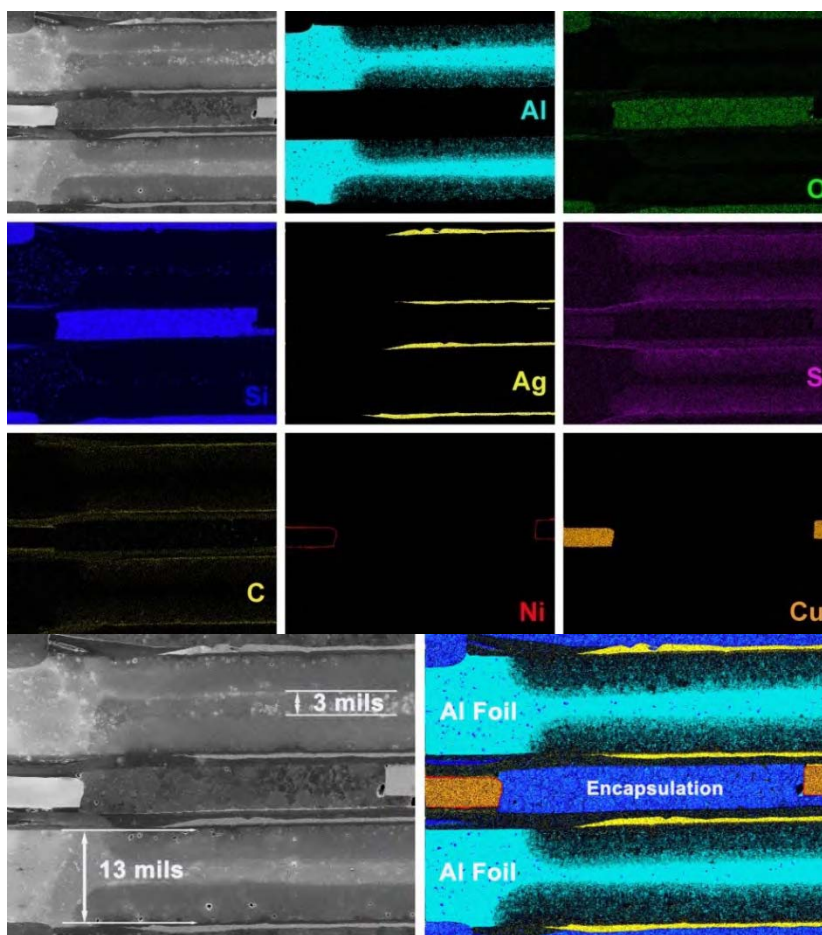
Figure 23. Cross-section SEM images and 2-dimensional EDX mapping results of a 100 \mu F, 6 V PA capacitor made by manufacturer E.
