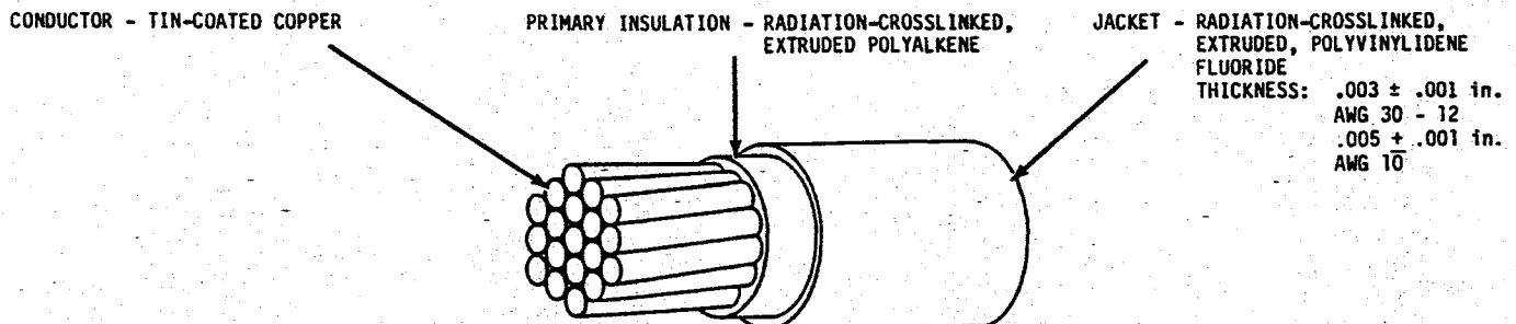
Figure 1 - Construction of Finished Wire
