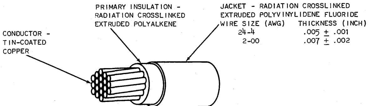
Figure 1 - Construction of Finished Wire
