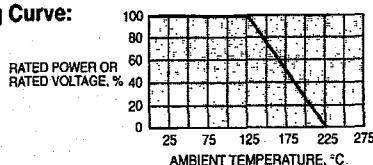
Figure 2. - Resistor derating.
