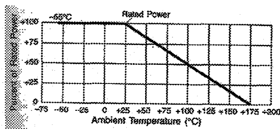
Figure 2. Derating .
