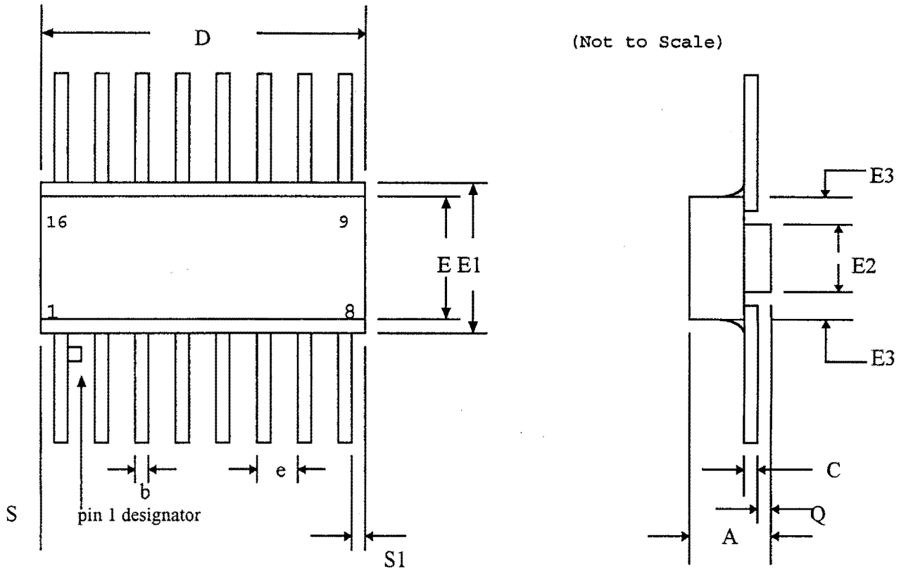
Figure 1 Package Outline
