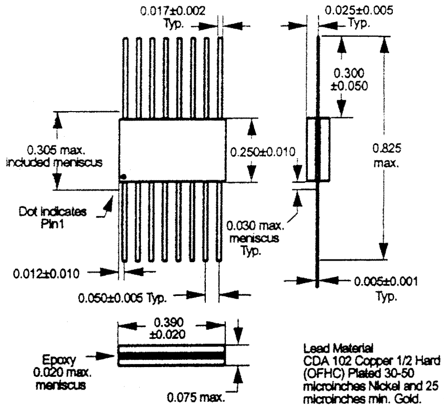
Figure 1. Package Outline.
