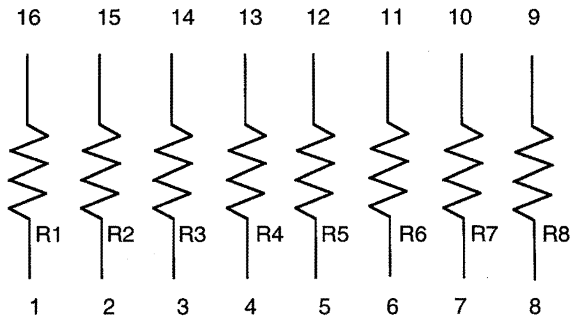
Figure 2. Device Schematic.
