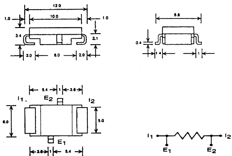
Figure 1. Package Outline.
