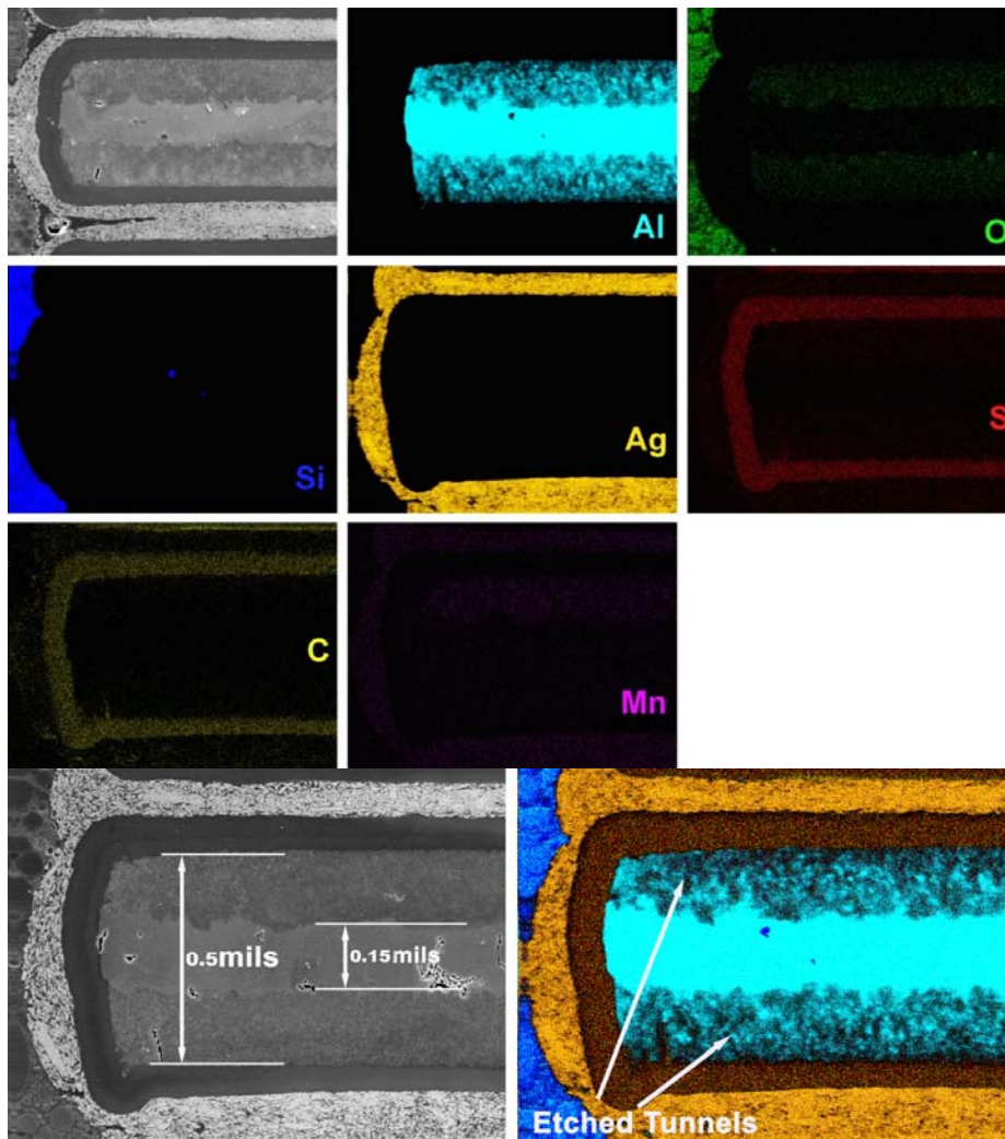
Figure 2. Two-dimensional EDX mapping results and cross-section SEM images show the end of single foils from the stack at high magnification for a 180 \mu\text{F} , 6.3V PA capacitor made by manufacturer A.
