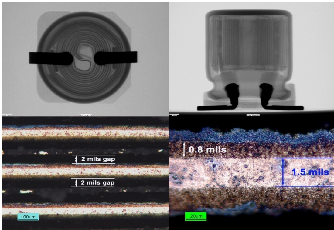
Figure 6. Radiographic images and high-magnification cross-sectional optical views of a 100 µF, 10 V PA capacitor made by manufacturer C show a traditional “wound” structure.
