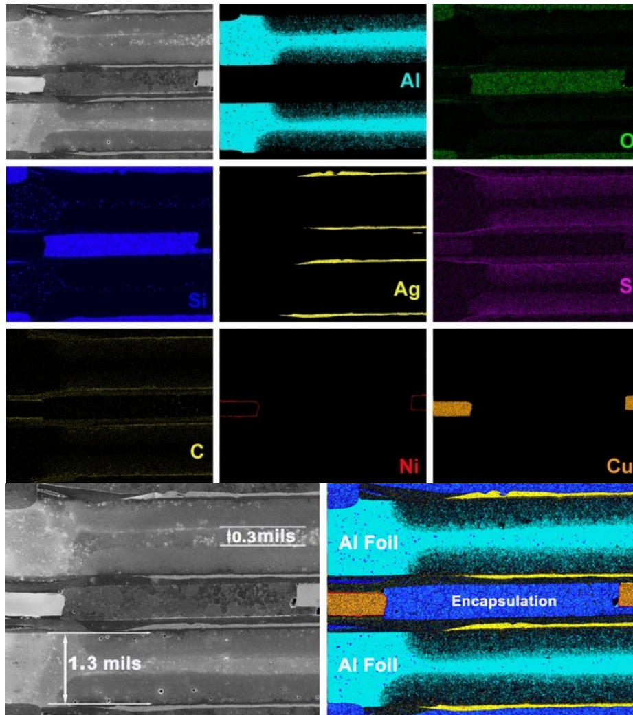
Figure 4. Two-dimensional EDX mapping results and cross-section SEM images of a 100 \mu F, 6V PA capacitor made by manufacturer E show a “laminated” structure.
