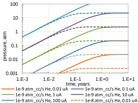
Figure II.3.1. Variations of pressure in a wet tantalum capacitor with volume 1 \text{cm}^3 at different levels of leakage currents and the measured leak rate of 10^{-8} atm*cc/s He (dashed lines) and 10^{-9} atm*cc/s He (solid lines).
