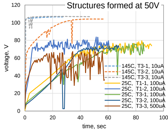
Figure III.5.3. Constant current stress testing for test structures after different conditioning: 145 °C, 50V for 30 hours (dashed lines) and 350 hours (SN1 and SN2) and 250 hours (SN3) at 50V at room temperature (solid lines).
