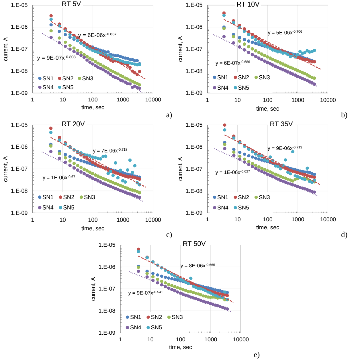
Figure III.3.8. Post high-temperature testing of leakage currents at room temperature and different voltages. For all samples anodes were in the downward positions.
