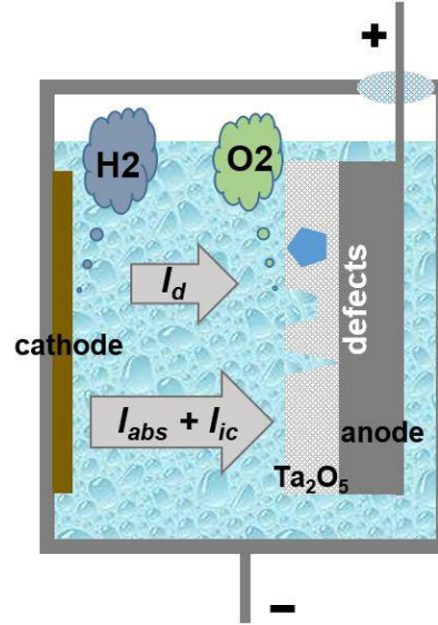
Figure II.2.1. A simplified schematic of a gas generation process in a case of wet tantalum capacitor.
