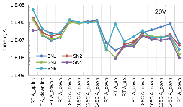
Figure III.3.7. Variation of currents at 20 V (a) and 50 V (b) through the testing.
