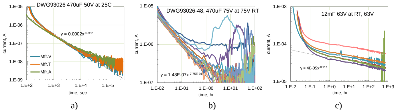
Figure I.8.1. Variations of leakage currents with time in different types of wet tantalum capacitors.
