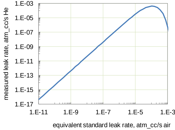
Figure.II.2.3. Measured leak rate, R_I vs. the standard leak rate, L , calculated per Eq.(8).
