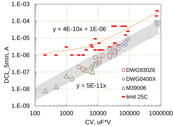
Figure I.5.1. Variations of experimental and specified values of DCL measured after 5 min of electrification with CV for wet tantalum capacitors. Red marks show the specified limits for the parts.
