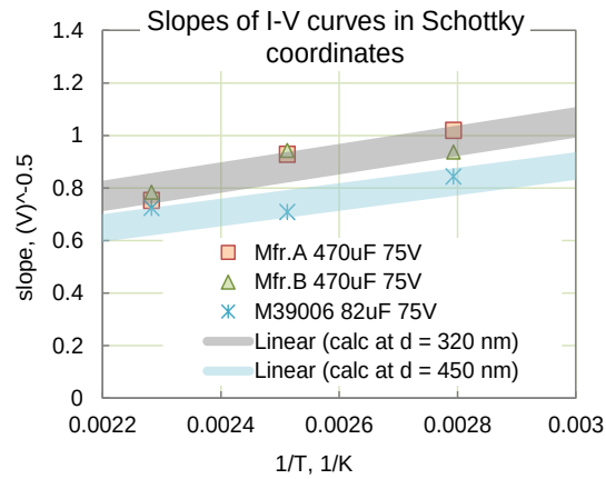
Figure I.7.2. Variation of slopes of the I - V curves in Schottky coordinates with temperature. Wide stripes are calculated slopes per the Simmons model, Eq.(I.7.1)
