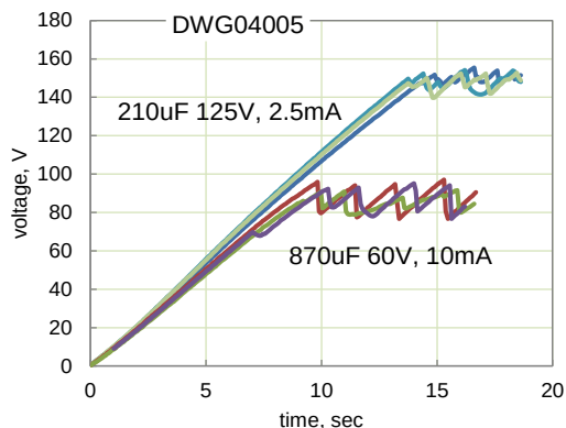
Figure I.2.1. Variations of voltage across three samples of 210 \mu F 125 V and 870 \mu F 60V DLA DWG04005 capacitors.
