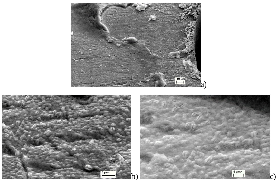
Figure III.4.3. An overall view of the surface of the tube (a) and close-up views of the oxide (b, c)
