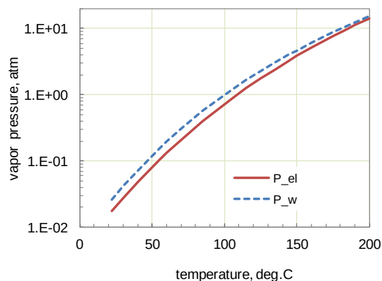
Figure II.1.1. Variations of saturated vapor pressure above 35% solution of H 2 SO 4 in water and above pure water.
