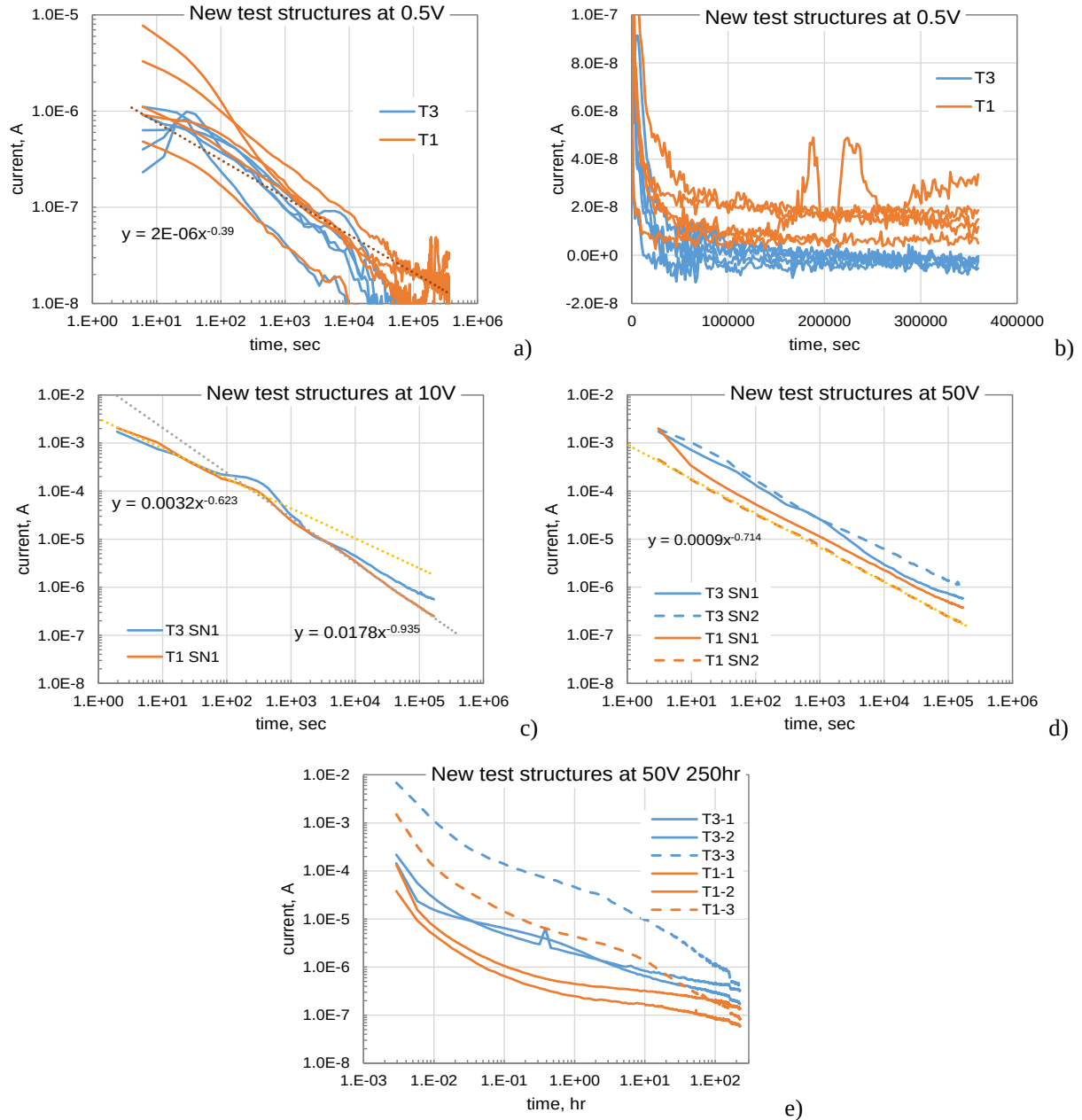
Figure III.3.9. Leakage currents in new test structures prepared in cases T3 and T1 during 100 hour testing consequently at 0.5 V (a and b), 10 V (c), and 50 V (d). Additional testing at 50 V for 250 hours is shown in figure e). Dashed lines correspond to virgin samples that had been tested at 0.5 V only. Note that figures a) and b) show variations of leakage currents with time in double logarithmic (a) and linear (b) coordinates. All samples were tested in the upward positions of anode terminals.
