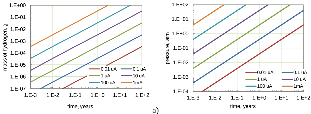
Figure II.2.2. Mass of hydrogen released by the electrochemical decomposition of electrolyte (a) and increase in pressure in a 1 cm 3 case (b) calculated at different levels of leakage current.
