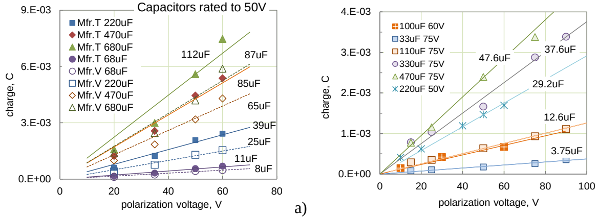
Figure I.4.1. Correlation between the absorbed charge and polarization voltage for capacitors from different manufacturers rated to 50 V (a) and for different part types (b).
