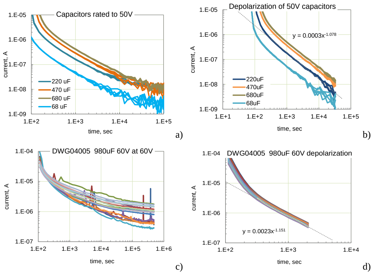
Figure I.8.1. Variations of leakage currents with time in different types of wet tantalum capacitors.
