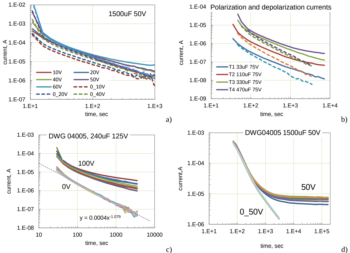
Figure I.3.1. Relaxations of polarization (solid lines) and depolarization (dashed lines) currents in different part types: a) 1500 \mu F 50 V capacitors at different voltages; b) different types of capacitors rated to 75 V; c) 10 samples of 240 \mu F 125 V capacitors tested at 100 V; d) 12 samples of 1500 \mu F 50 V capacitors. Here and below, absolute values of depolarization currents are shown as dashed lines.
