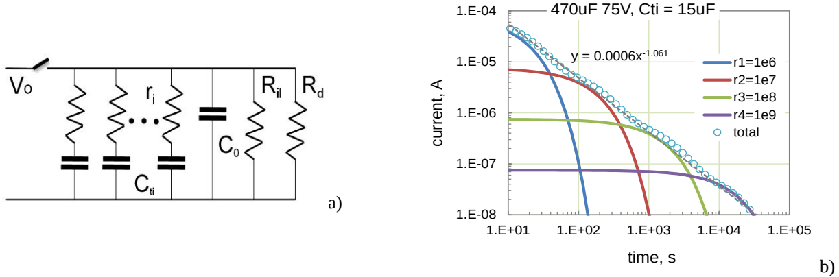
Figure I.6.2. An equivalent circuit for modeling leakage currents in wet tantalum capacitors (a) and simulation of absorption currents in a 470 \mu\text{F} 75 V capacitor for a case when i = 4 , C_{ti} = 15 \mu\text{F} , r_1 = 1\text{E}6 ohm, and r_{i+1} = 10 r_i
