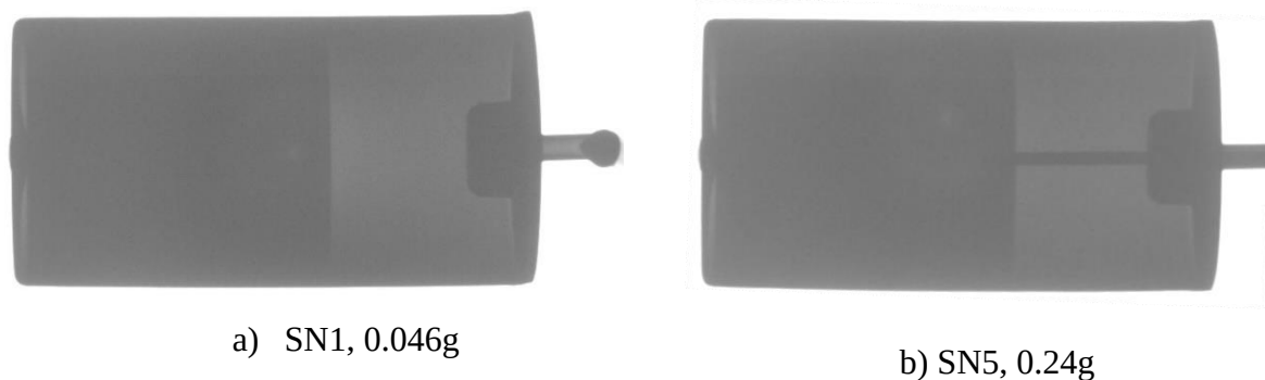
Figure III.2.1. X-ray views and amount of electrolyte in case T3 SN1 and SN5 model structures of wet tantalum capacitors. The amount of electrolyte in other samples was ~ 0.1 g.
