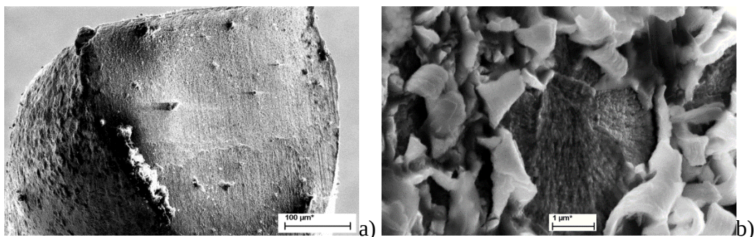
Figure III.4.2. Overall (a) and close-up (b) views of the tip of the wire.
