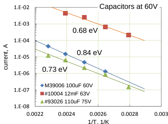
Figure I.7.4. Temperature dependence of leakage currents in different types of wet tantalum capacitors.
