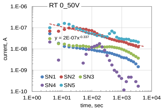
Figure III.3.5. Variations of leakage currents at room temperature and 35 V (a, b) and 50 V (c, d) for the upward position of anodes.
