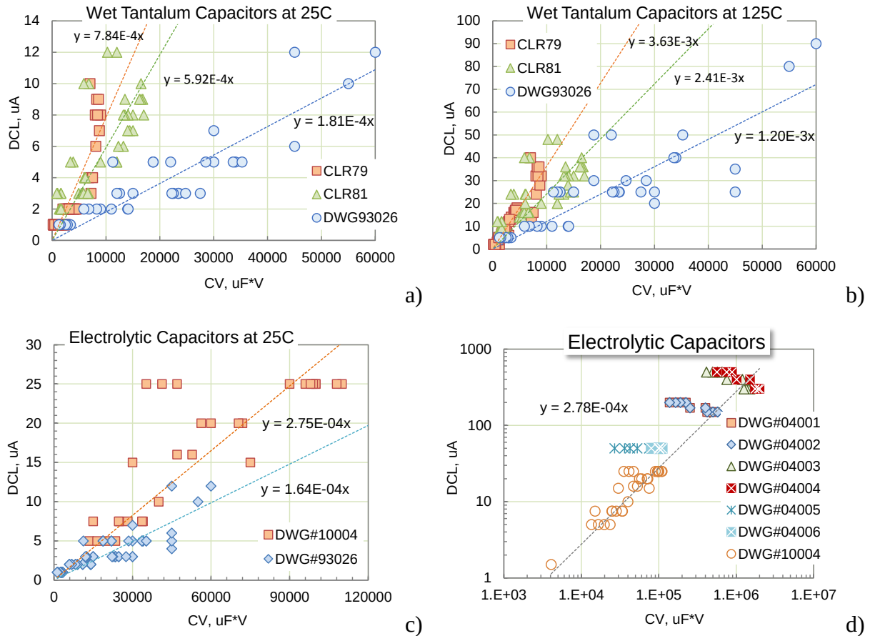
Figure I.1.3. Specified leakage currents for different types of wet tantalum capacitors. (a, b) CLR79, CLR81, and DLA DWG93026 at 25 °C (a) and 125 °C (b). c) Comparison between DLA DWG10004 and DLA DWG93026. (d) Large CV values capacitors per DLA DWG0400X and DLA DWG 10004.
