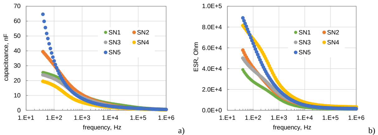
Figure III.5.2. Frequency dependencies of capacitance (a) and ESR (b) in the model structures after the testing.
