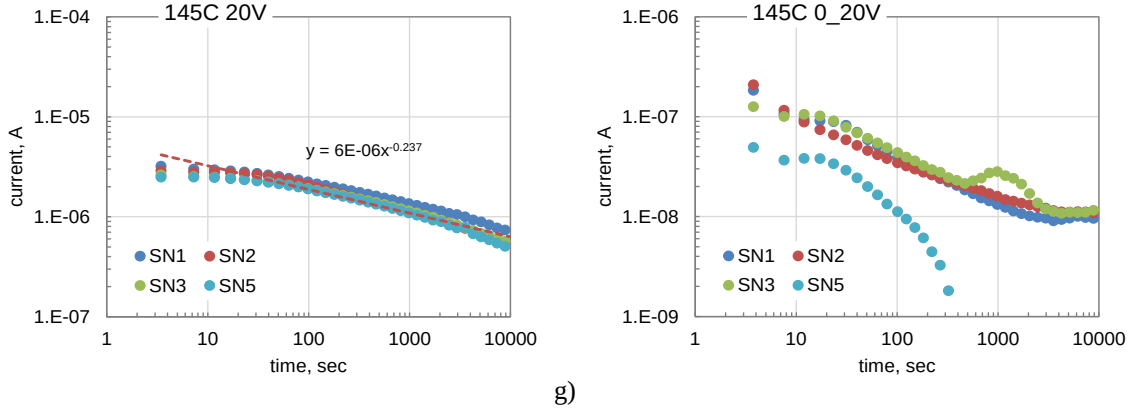
Figure III.3.2. Variations of currents with time during polarization (20 V) and depolarization (0_20 V) cycles at different temperatures.
