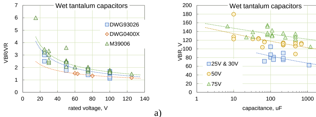
Figure 1.2.2. Variations of the normalized breakdown voltages with the nominal rated voltage (a) and dependence of VBR on capacitance for capacitors rated to different voltages (b).
