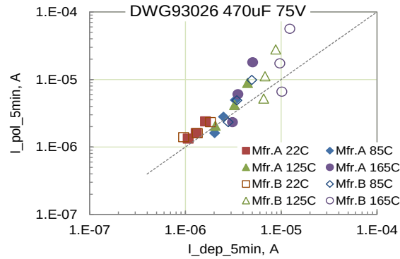
Figure I.3.2. Correlation between polarization and depolarization currents measured after 300 sec at different temperatures for 470 \mu\text{F} 75 V capacitors from two vendors.
