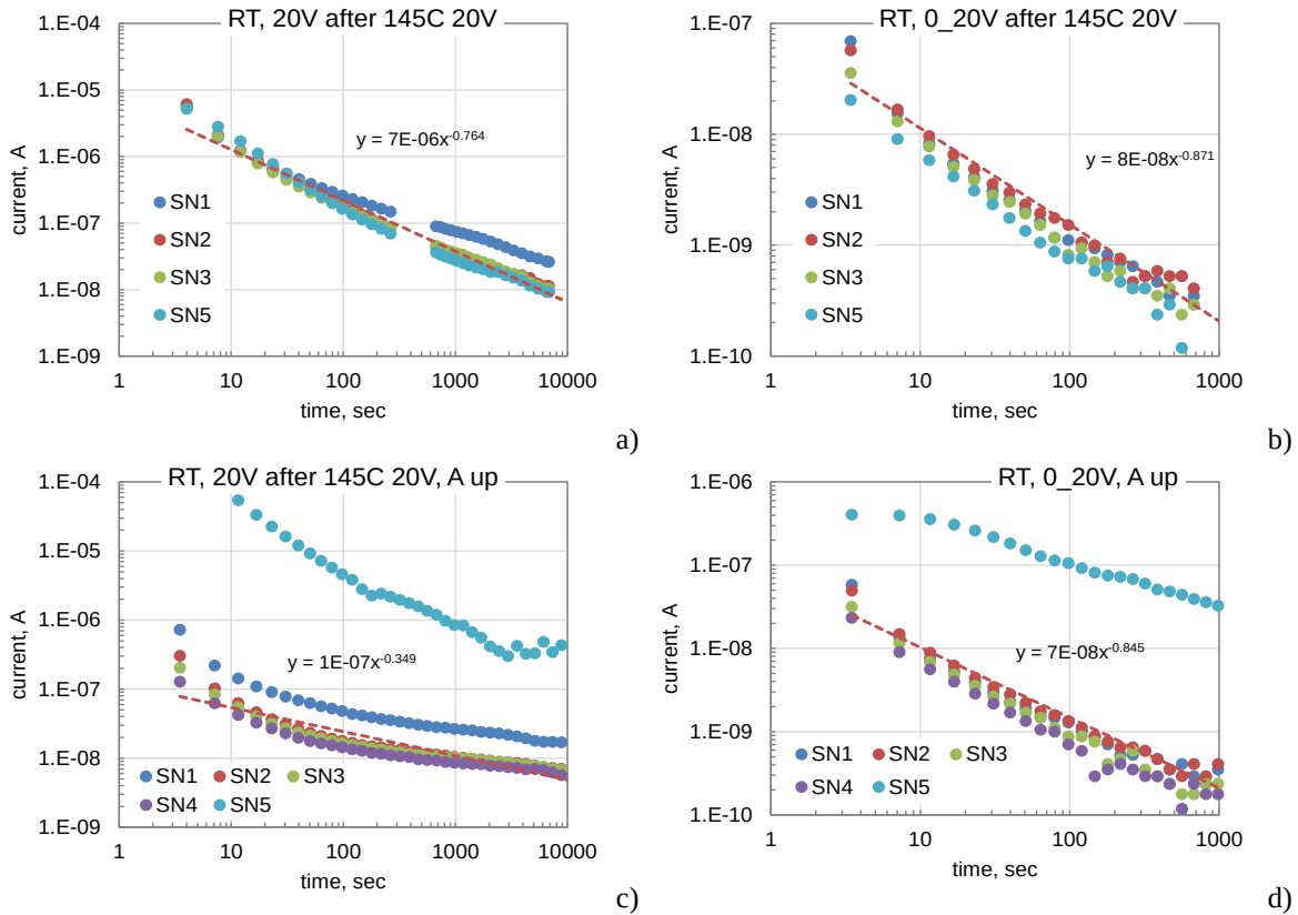
Figure III.3.3. Post 145 °C testing measurements at room temperature and 20V first at downward (a, b) and then at upward (c, d) anodes positions.
