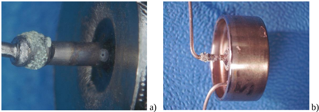
Figure III.3.4. Weld corrosion and electrolyte leak in SN4 after 145 °C testing (a) and an example of a leak failure in a button-style capacitor (b).
