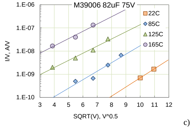
Figure I.7.1. Variations of leakage currents with square root of voltage for different types of wet tantalum capacitors.
