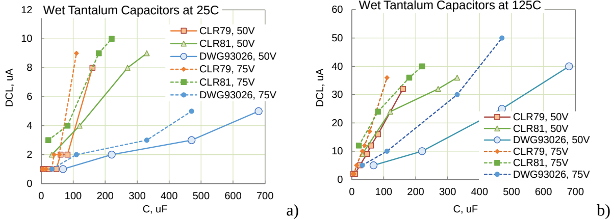
Figure I.1.1. Variation of maximum specified leakage currents with capacitance at 25 °C (a) and 125 °C (b) for capacitors rated to 50 V and 75 V.
