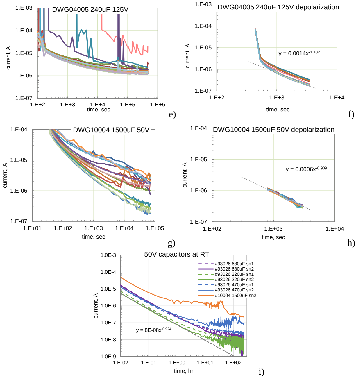
Figure I.8.2. Long-term variations of leakage currents at room temperature under rated voltages (a, c, e, g, i) and depolarization currents (b, d, f, h) in different types of wet tantalum capacitors.
