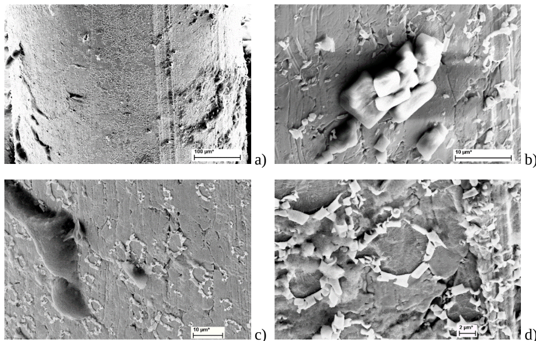
Figure III.4.1. Oxide and contaminations on the surface of wire. a) overall view, b) sulfur crystals (d), composition of S/O/C, and c) close-up views of broken oxide on the surface. Estimations showed that the thickness of the oxide is ~ 150 nm.
