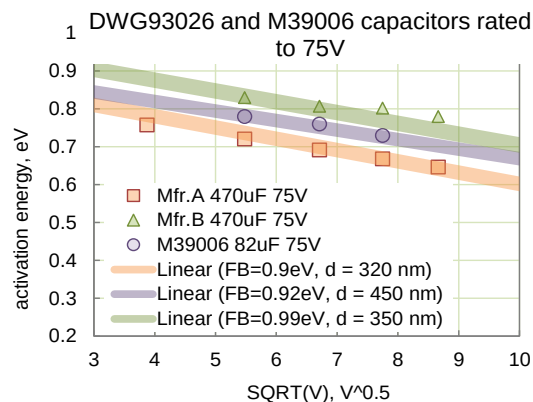
Figure I.7.5. Voltage dependence of activation energy. Wide stripes are results of calculation per Eq.(I.7.2).
