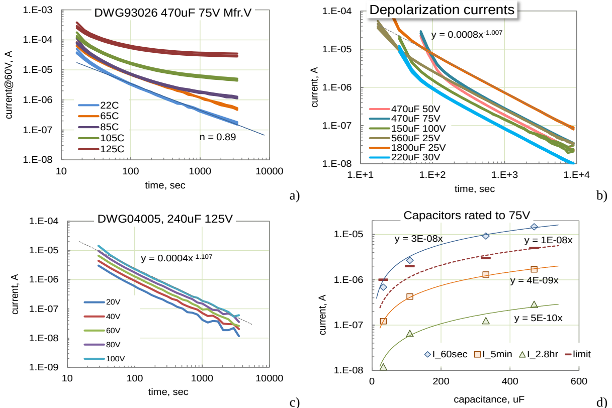
Figure I.3.3. Relaxation of absorption currents during 1 hour for different types of capacitors.
