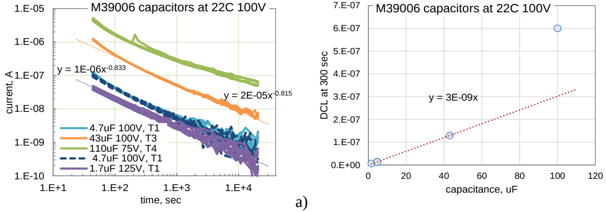
Figure I.3.5. Relaxation of polarization currents in different types of M39006 capacitors (8 to 10 samples in a group) (a) and a variation of DCL measured after 5 min of electrification with the value of capacitance (b).
