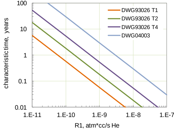
Figure II.3.3. Characteristic times for pressure build-up for different types of capacitors.
