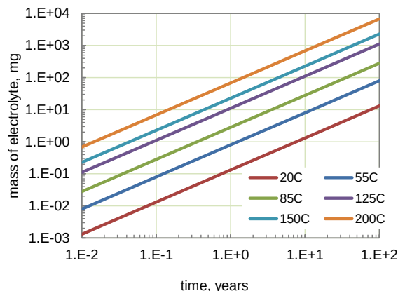
Figure II.1.3. Amount of electrolyte escaped at different temperatures from a capacitor having a measured helium leak rate of 10^{-8} atm*cc/s.
