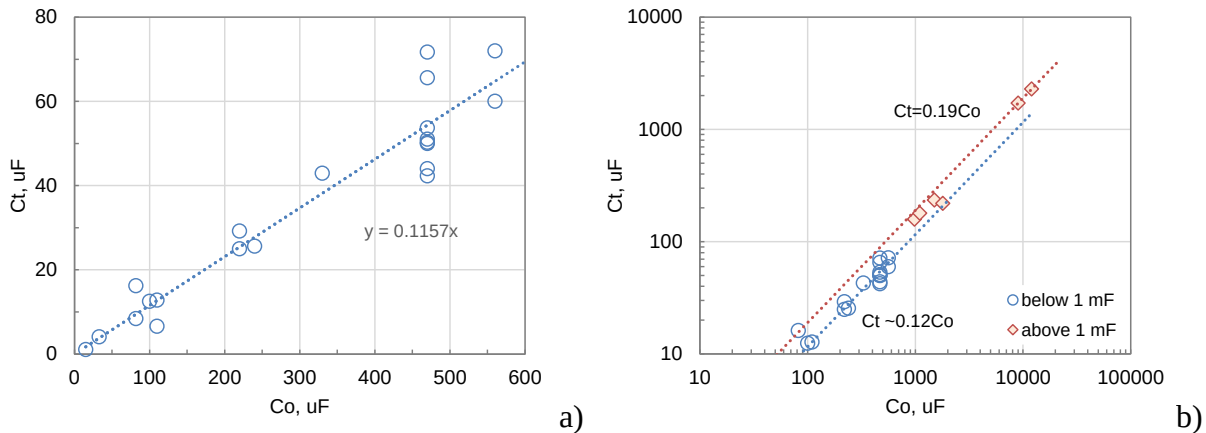
Figure I.4.2. Correlation between absorption and nominal capacitance for capacitors below 560 \mu\text{F} (a) and for all types of tested capacitors (b).
