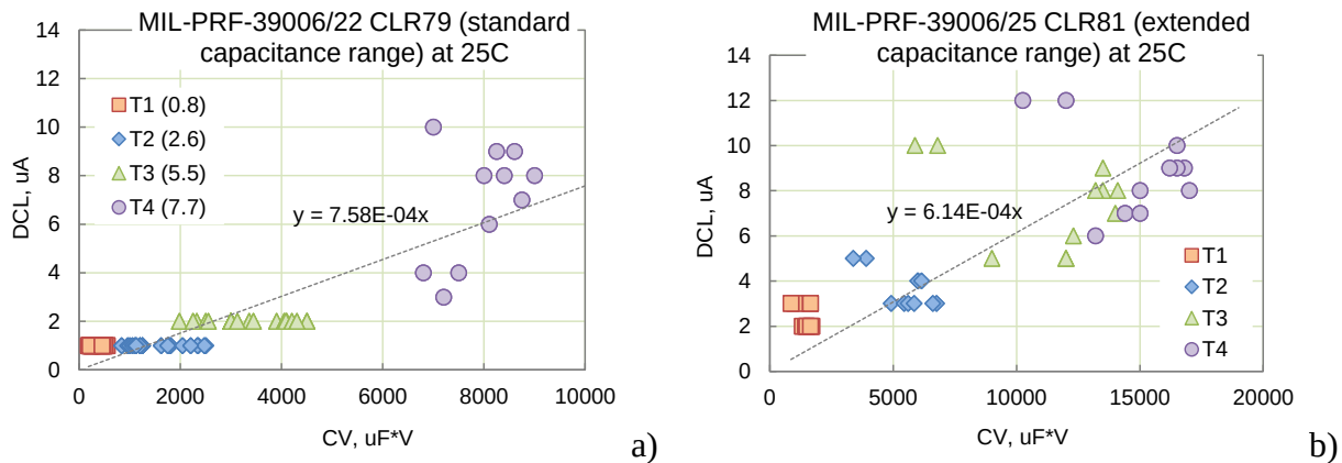
Figure I.1.2. Correlation between the specified levels of DCL and CV values for CLR79 (a) and CLR81 (b) capacitors. Different marks correspond to different case sizes, from T1 to T4.
