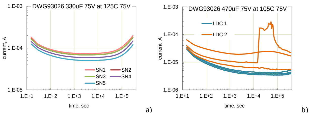
Figure I.8.3. Variations of leakage currents with time at high temperatures. a) DLA DWG93026, 330 \mu\text{F} 75 V capacitors during 100-hour HALT at 125^\circ\text{C} and 75 V. b) Two lots of DLA DWG93026, 470 \mu\text{F} 75 V capacitors during 100-hour HALT at 105^\circ\text{C} and 75 V. Note that samples with LDC1 are virgin and with LDC2 are after qualification testing.
