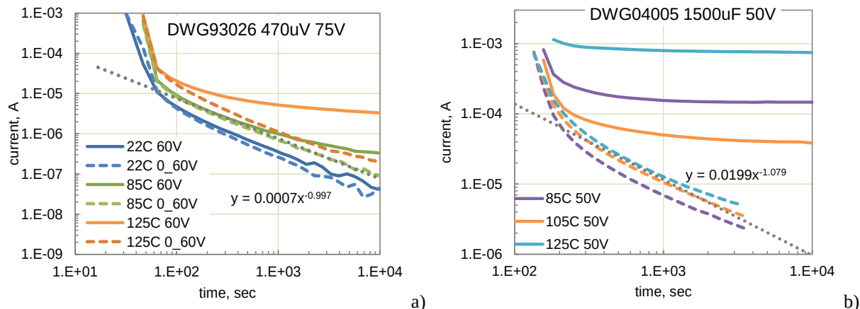
Figure I.3.4. Relaxation of polarization and depolarization currents at different temperatures for 470 \mu F 75 V (a) and 1500 \mu F 50 V (b) capacitors.
