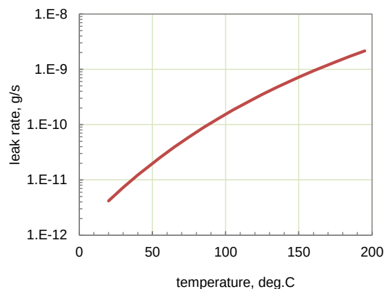
Figure II.1.2. Variation of the electrolyte leak rate with temperature for a case with the measured leak rate 10^{-8} atm*cc/s He.
