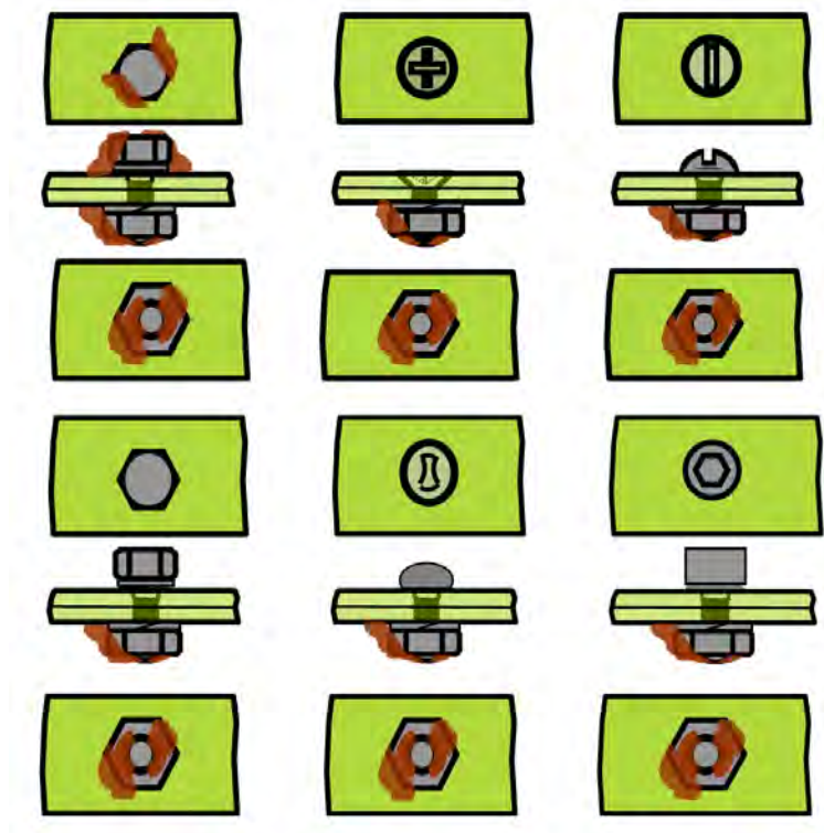
Figure 9-8. Locking of Screws and Bolts with Nuts
