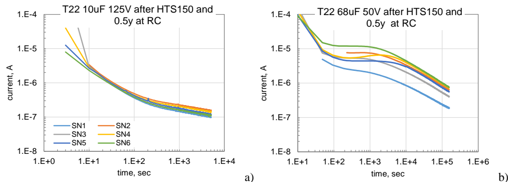
Figure 17. Relaxation of leakage currents at rated voltages for 10 \mu F 125 V (a) and 68 \mu F 50 V (b) capacitors after HTS150 and 0.5 year of storage at room conditions.
