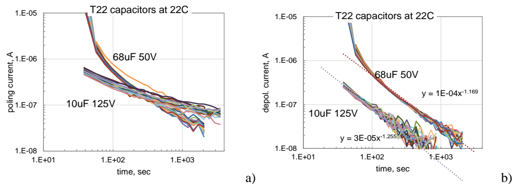
Figure 9. Polarization (a) and depolarization (b) currents for 20 samples of 10 \mu\text{F} 125 V and 68 \mu\text{F} 50 V capacitors.
