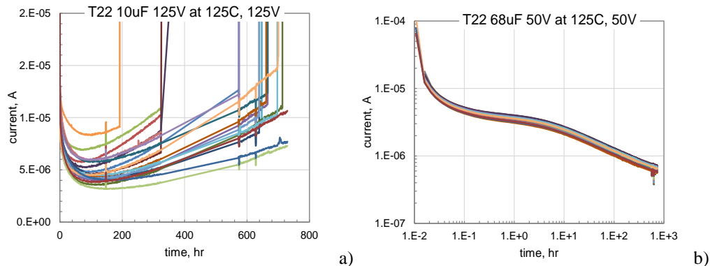
Figure 20. Variations of leakage currents with time during HALT at 125 °C and rated voltages for 10 \mu\text{F} 125 V (a) and 68 \mu\text{F} 50 V (b) capacitors.
