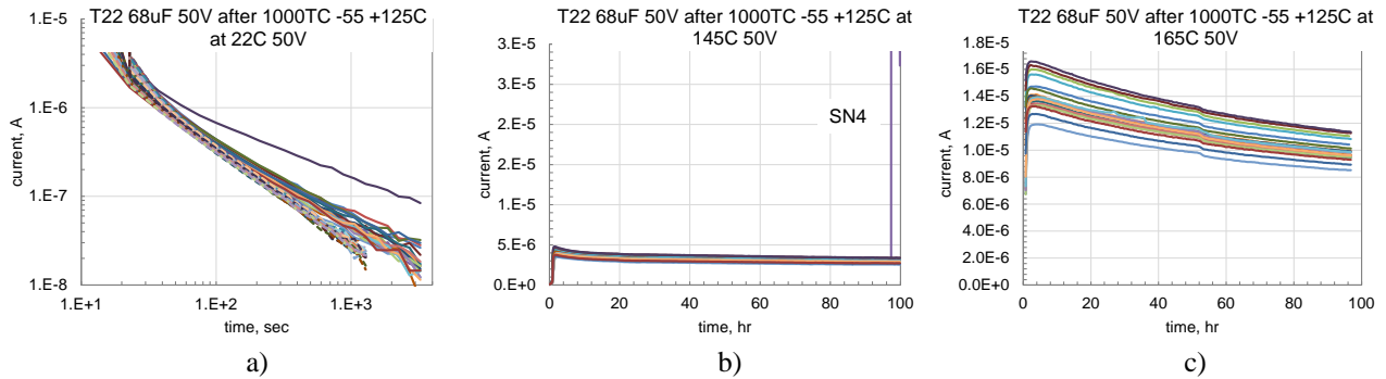
Figure 21. Leakage currents in 20 samples of 68 \mu\text{F} 50 V capacitors after 1000 temperature cycles between -55\text{ }^{\circ}\text{C} and +125\text{ }^{\circ}\text{C} . a) relaxation of leakage currents at room temperature (solid lines indicate polarization, and dashed lines depolarization currents). b) HALT at 145\text{ }^{\circ}\text{C} , 50 V for 100 hours. c) HALT at 165\text{ }^{\circ}\text{C} , 50 V for 100 hours.
