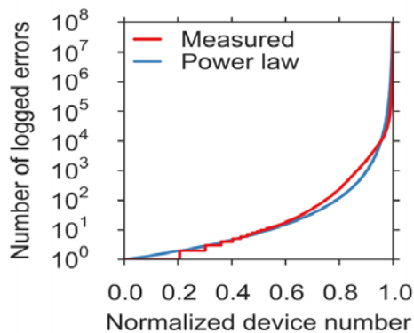
Figure 10: Memory Error Distribution – Power-Law (Facebook)
