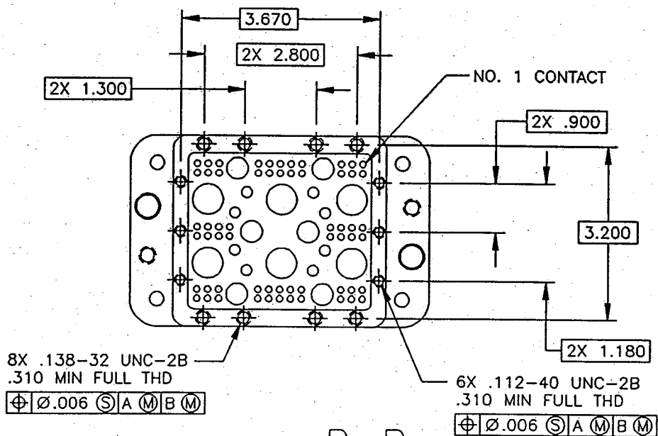
VIEW B-B (-1)
