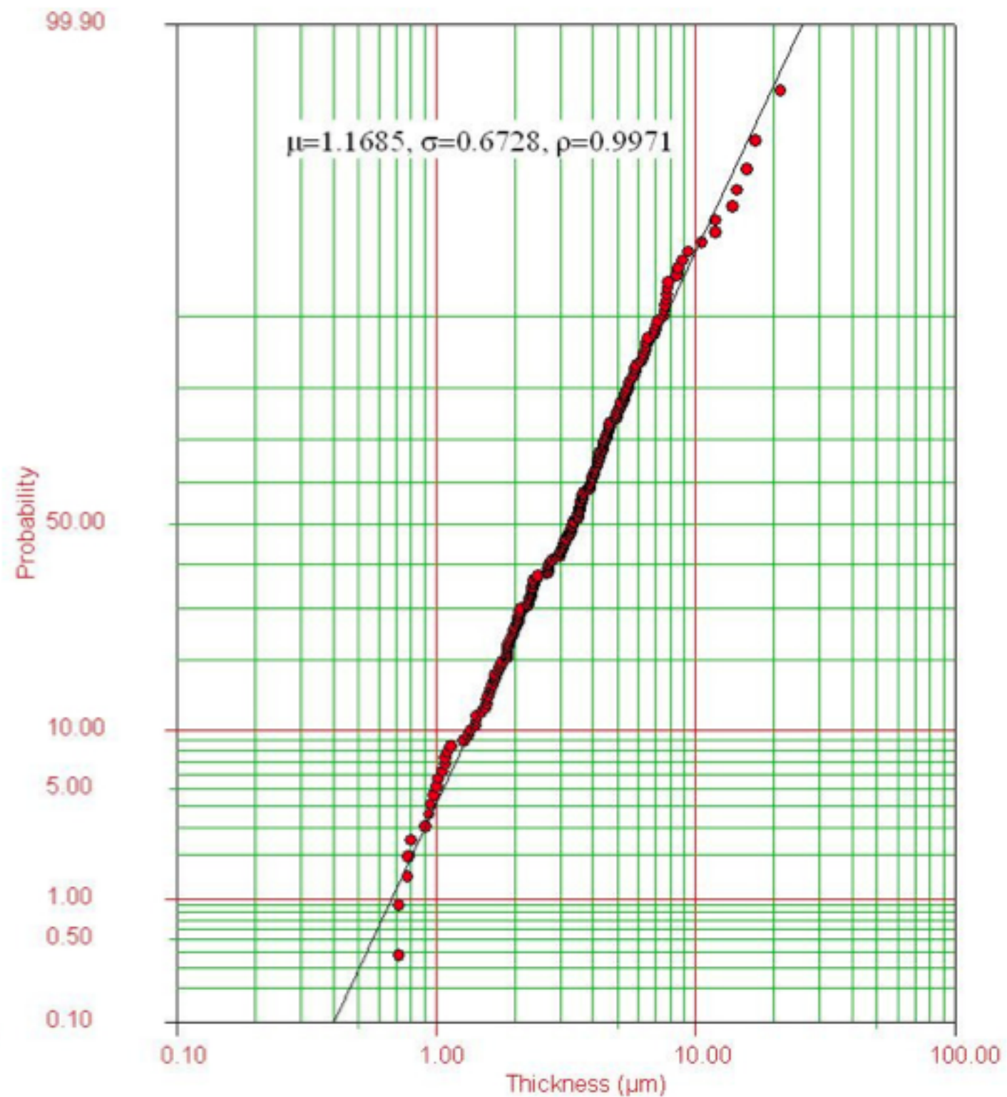
Figure 60 Lognormal cumulative probability distribution of whisker thicknesses for Set 2
