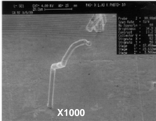
Figure 5. Tin Whiskers on the Non-conformally Coated Side
