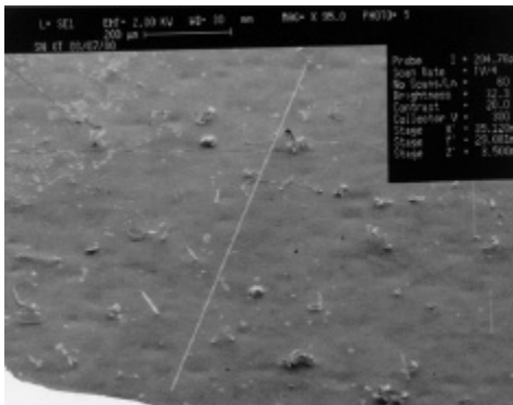
Figure 13. Tin Whiskers of the Non-conformally Coated Side (x95)
